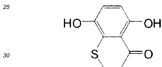
Synthetic Monomer 13
