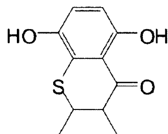
Synthetic Monomer 14
