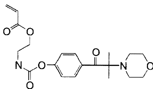
Synthetic Monomer 12
