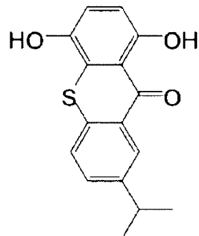
Synthetic Monomer 16
