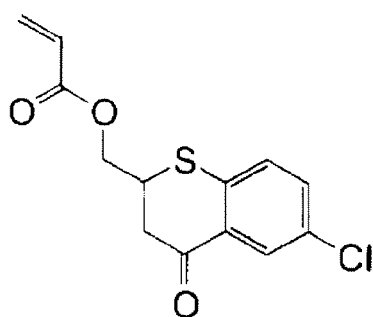
Synthetic Monomer 8
