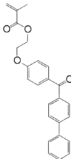
Synthetic Monomer 7
