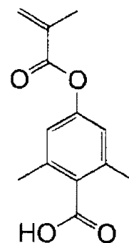
Synthetic Monomer 10
