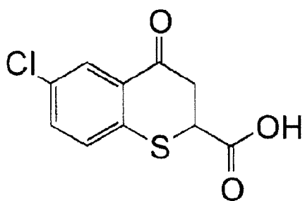
Compound B
