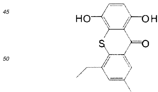
Synthetic Monomer 15
