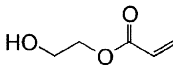
Compound C
