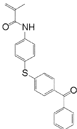
Synthetic Monomer 5
