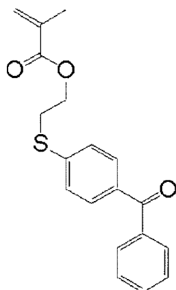
Synthetic Monomer 6
