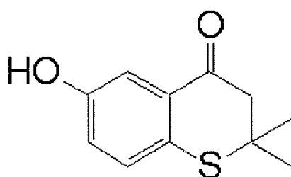
Compound A
