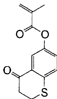
Synthetic Monomer 9
