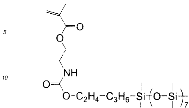
Synthetic Monomer 11
