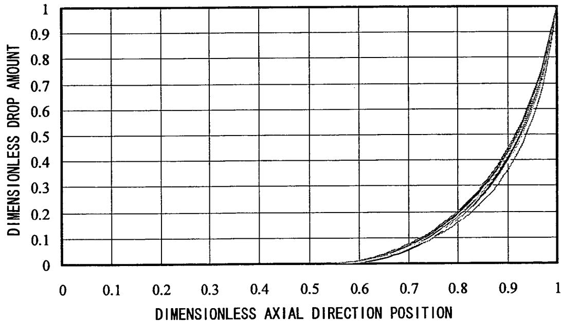
DIAGRAM OF DIMENSIONLESS CROWNING CURVE AT DESIGN LOAD OF 40%Cr
