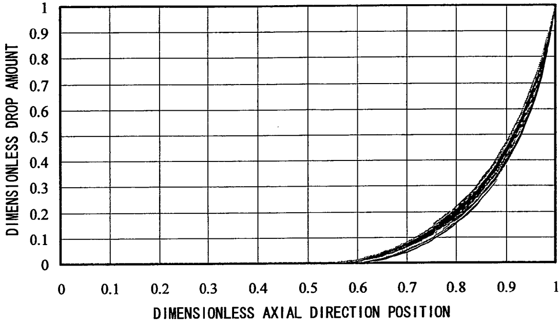
DIAGRAM OF DIMENSIONLESS CROWNING CURVE AT DESIGN LOAD OF 35%Cr
