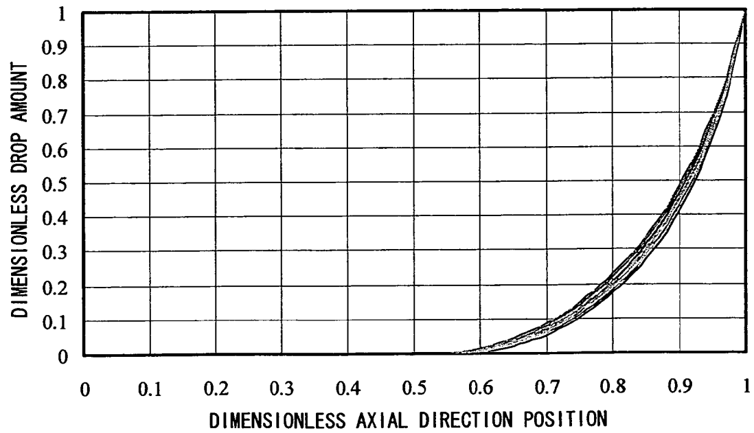
DIAGRAM OF DIMENSIONLESS CROWNING CURVE AT DESIGN LOAD OF 30%Cr
