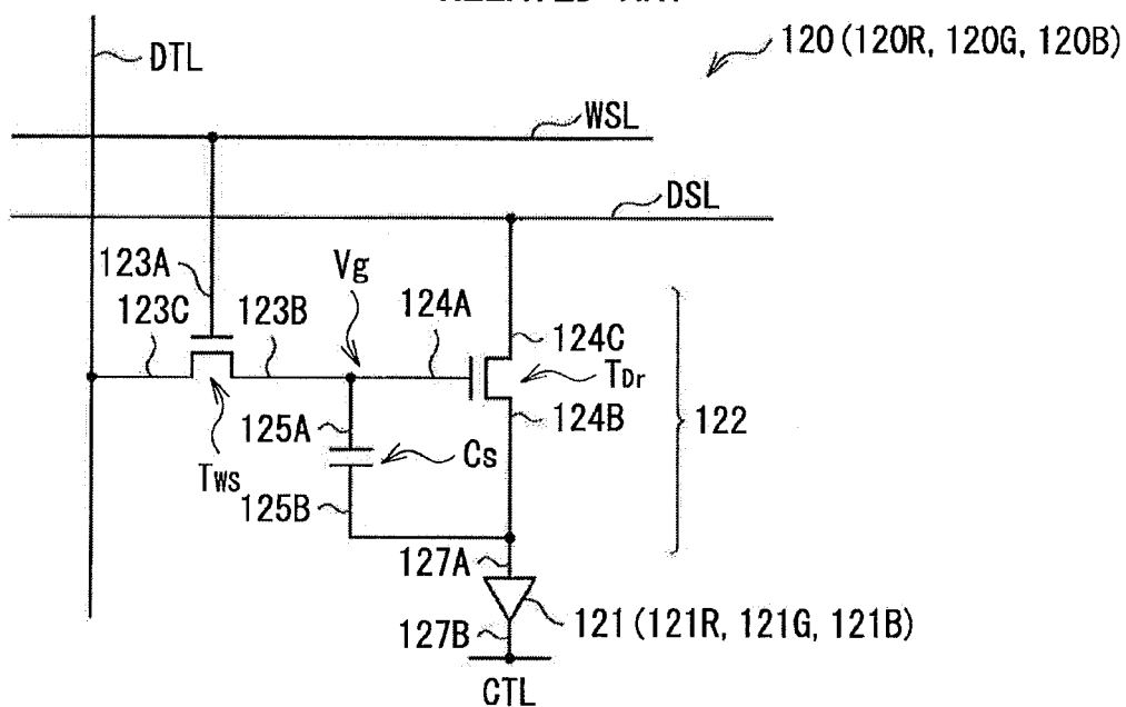
FIG. 16 RELATED ART
