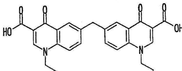
Compound (B6)
