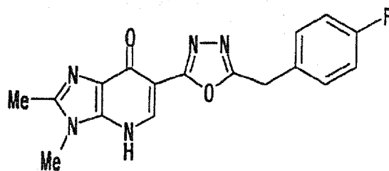
Compound (B2)
