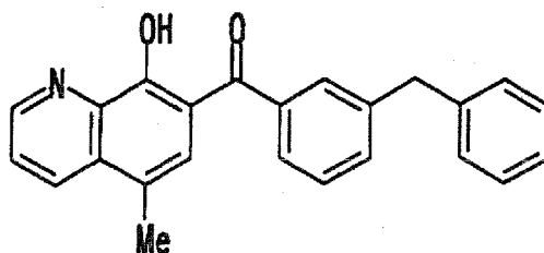
Compound (B3)
