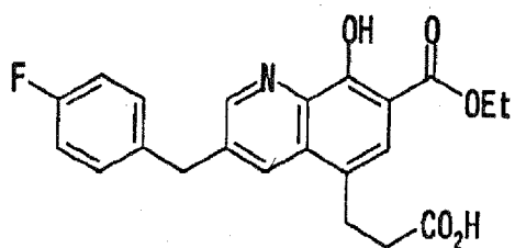
Compound (B1)
