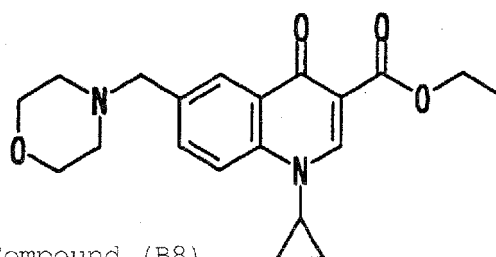
Compound (B8)
