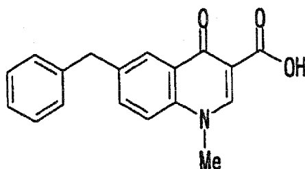
Compound (B7)
