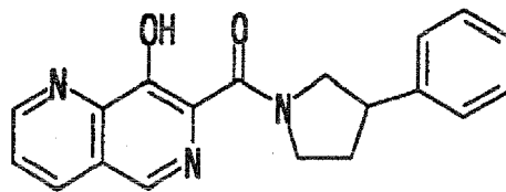
Compound (B4)
