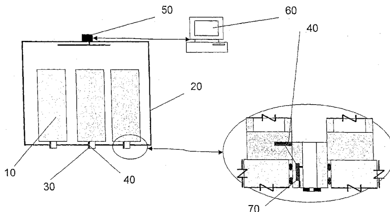
Figure 4: In- Situ Integrity Test Configuration Flow Sensor / RFID Communication Device within Multi-Element Filter Configuration
