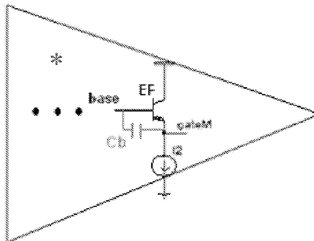
Emitter Follower Output Stage
