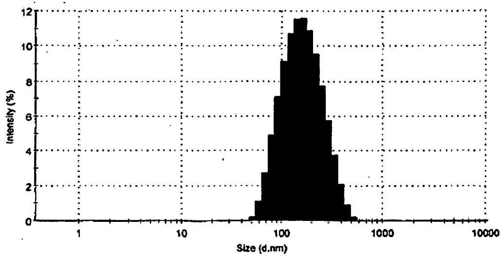
Figure 4 (a): Histogram showing particle size distribution of the nanodispersion of Example 9 at initial time
