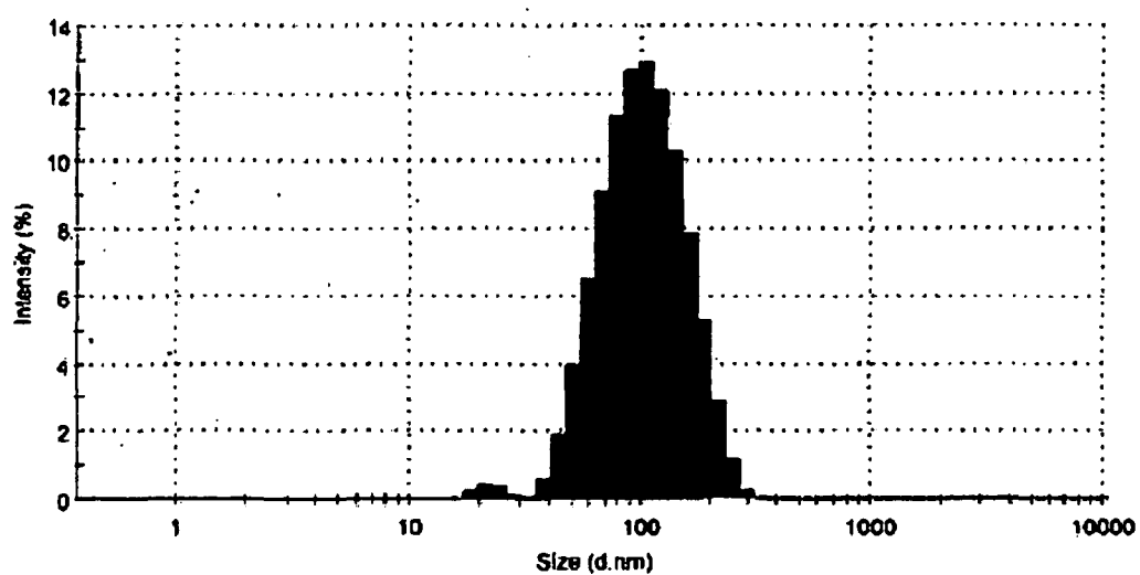
Figure 5 (b): The histogram showing the particle size distribution of the nanodispersion of docetaxel of Example 24 D when stored at room temperature for 8 hours.
