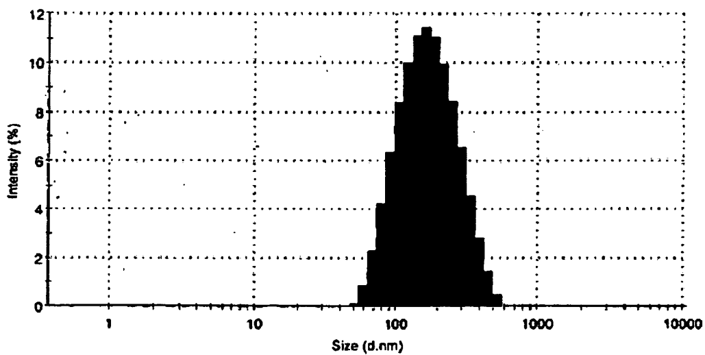
figure 4 (b): The histogram showing the particle size distribution of the nanodispersion of paclitaxel Example 9 when stored at room temperature for 24 hours
