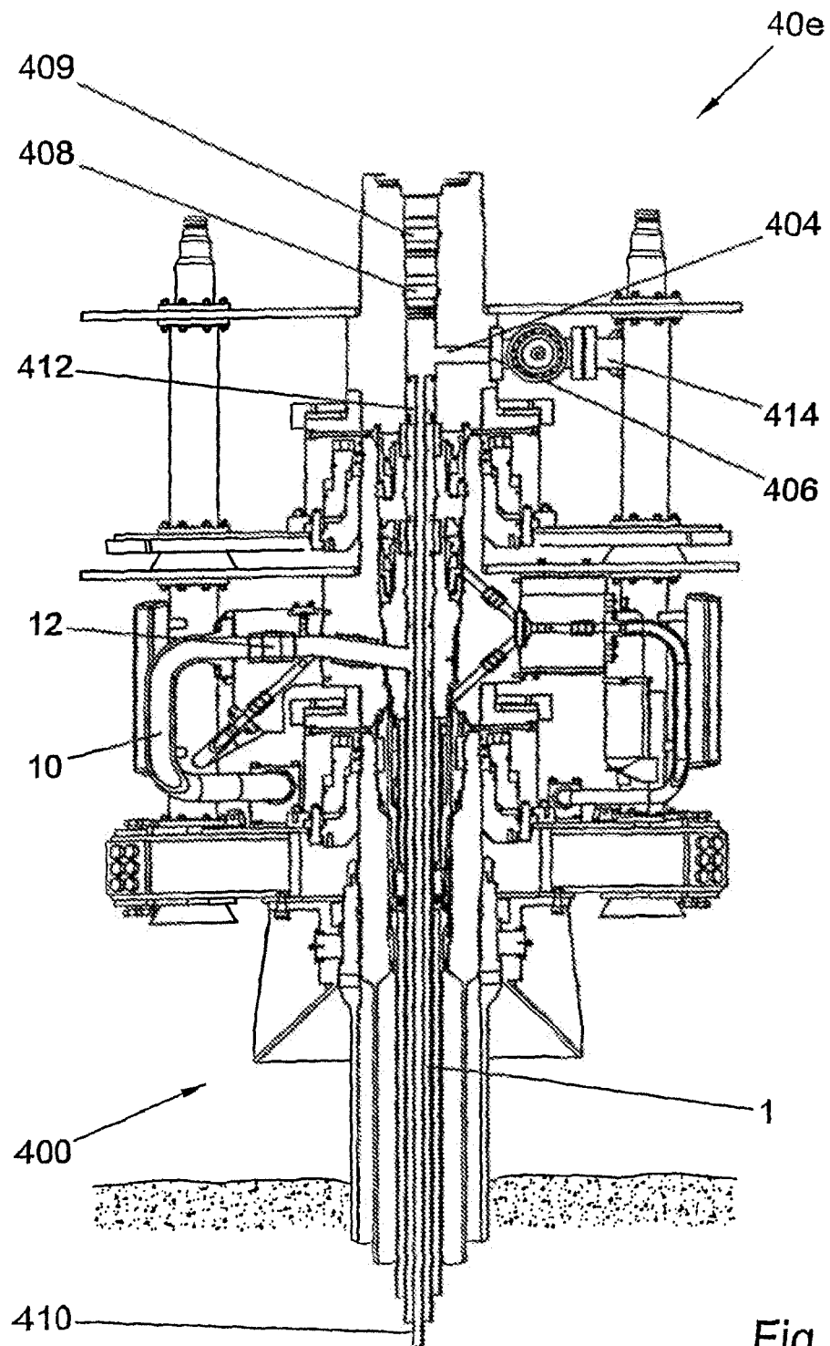
TYPICAL SECTION
