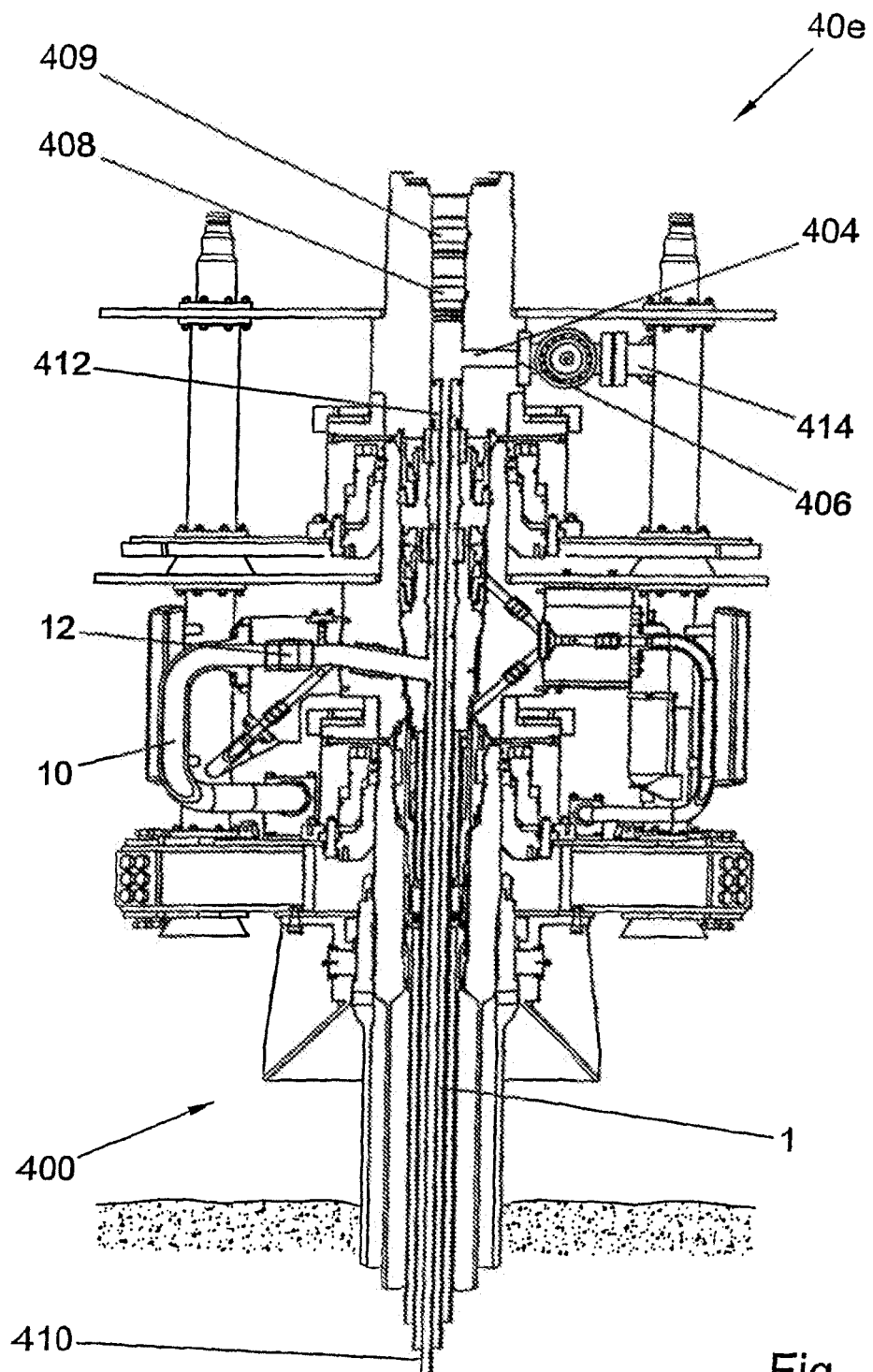
TYPICAL SECTION
