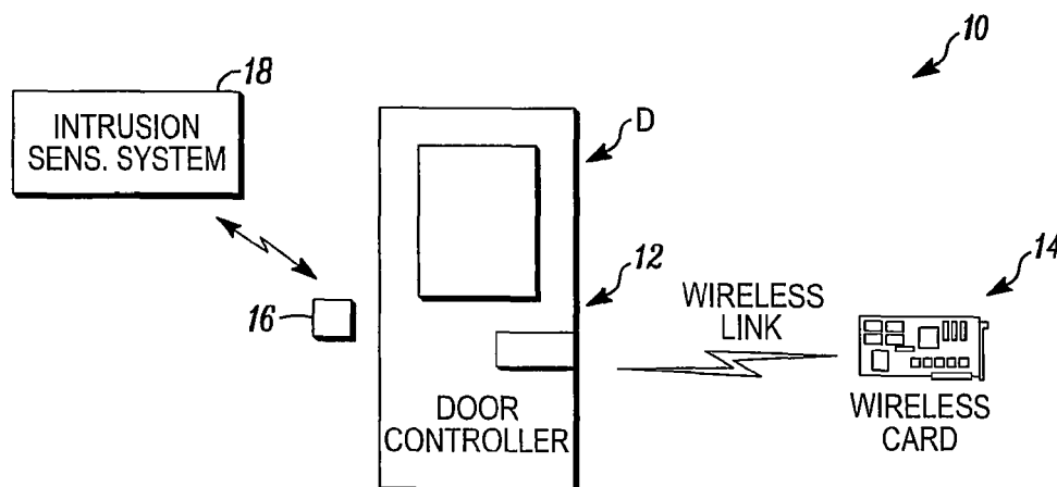
STAND-ALONE DOOR CONTROLLER SYSTEM
