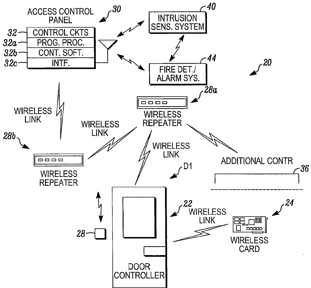
DOOR CONTROLLER SYSTEM WITH ACCESS CONTROL HOST
