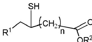
Formula IV
