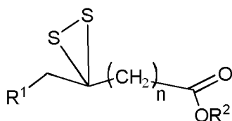
Formula V
