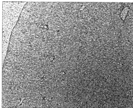
C4-SULFATASE ( \times 50 )
