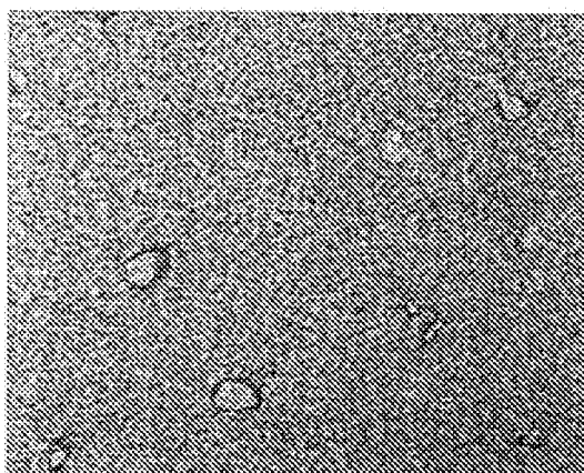
C4-SULFATASE ( \times 100 )
