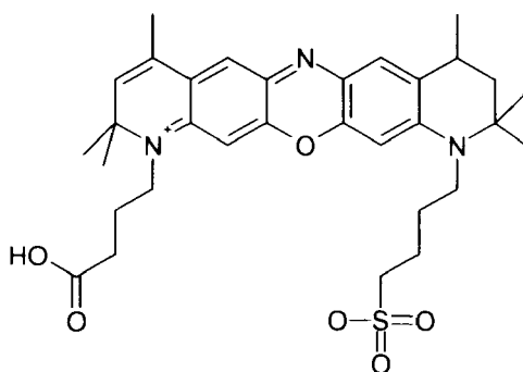
Structure of the JA286 dye
