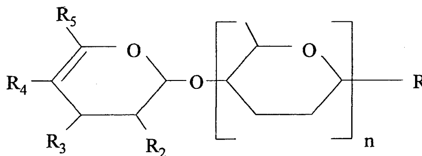
Fig. 2: Preferred terminal hexose acid group
