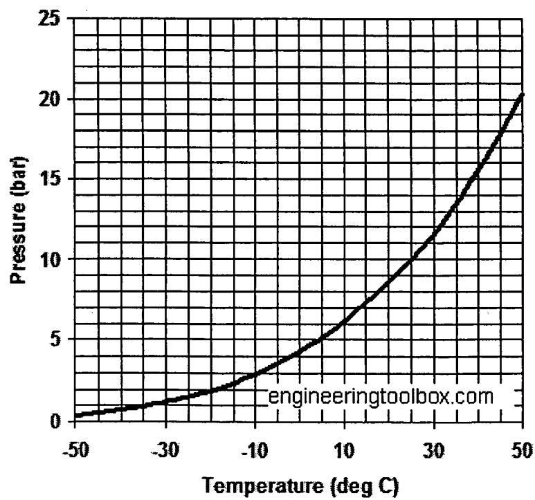
Evaporation Curve of Ammonia
