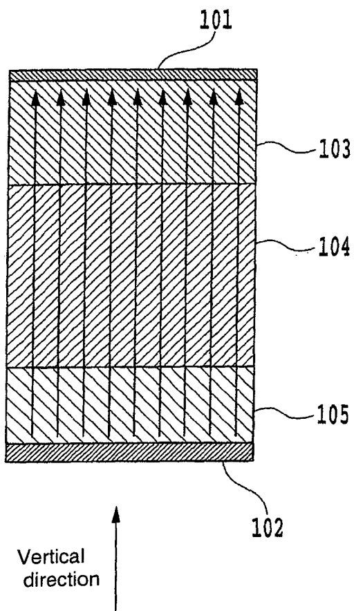
(a) Vertical device structure
