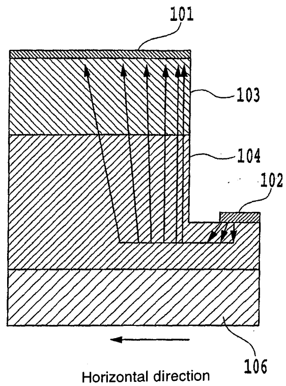
(b) Horizontal device structure
