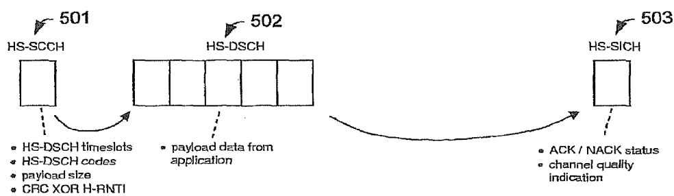
HSDPA frame structure
