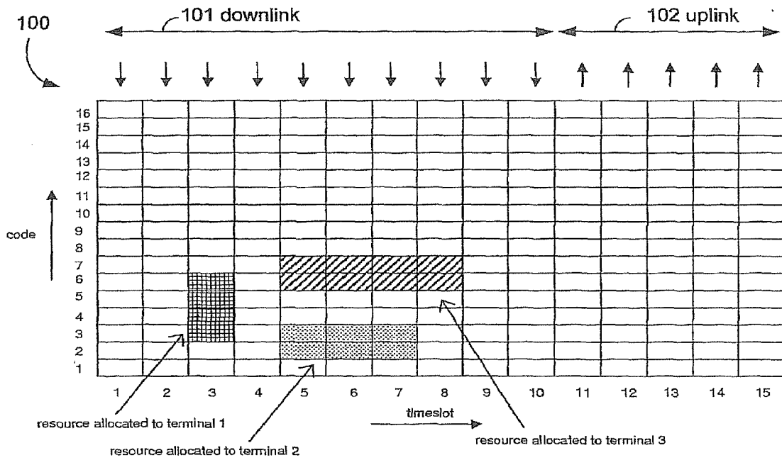
Typical TDD radio frame
