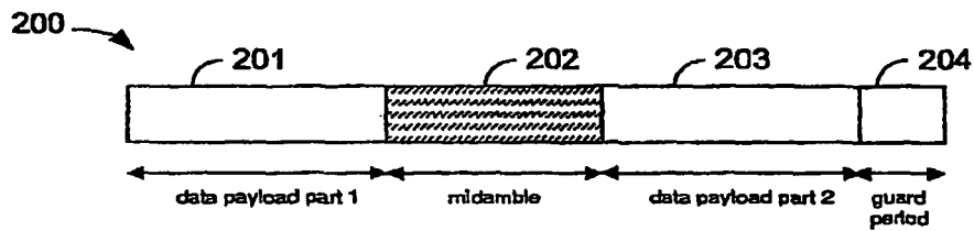
UTRA TDD timeslot configuration
