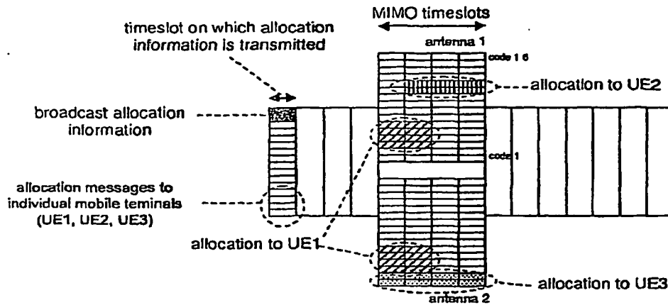
Example of broadcast code allocation information in UTRA TDD
