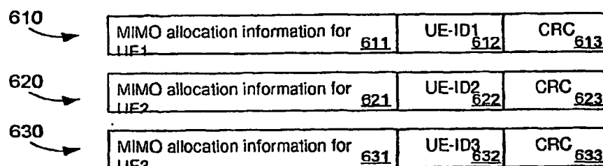
BS-SCCH structure for implicitly broadcasting allocation information
