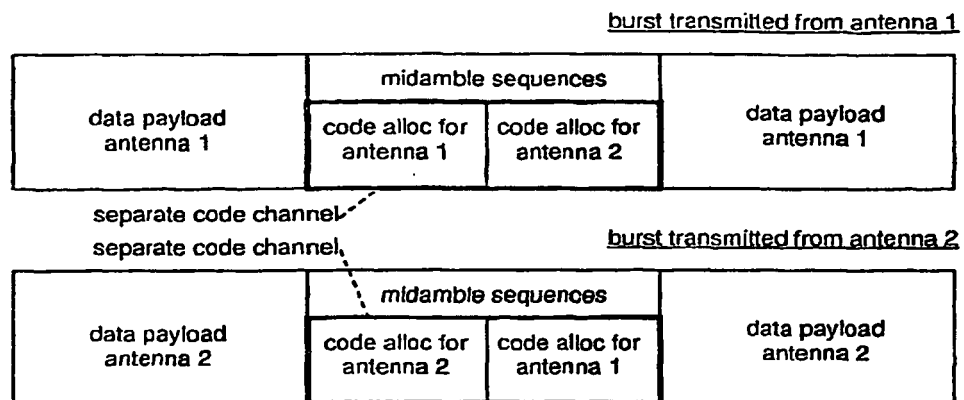
Broadcast transmission of code allocation information in midamble portion of burst
