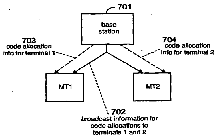
Broadcasting allocation information to terminals
