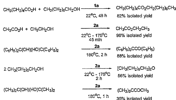
Scheme 1. Representative reactions using IL 1a and 2a .
