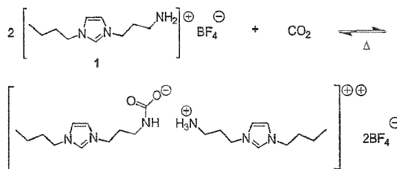
Scheme 2. Proposed reaction between TSIL 1 and CO 2 .
