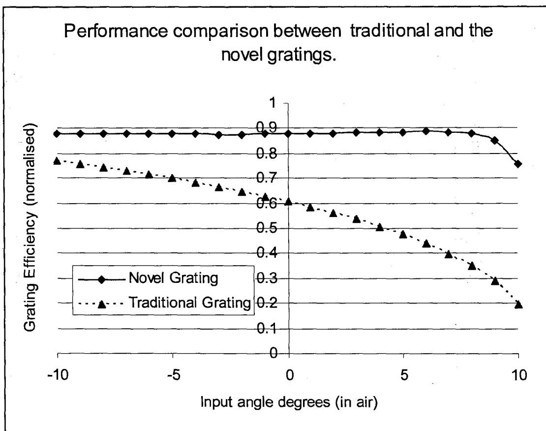
Figure 5 Graph comparing the angular bandwidth of the two types of gratings for the +1 reflected order. Input wavelength is 532nm.
