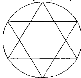
Squared Circle (SQC)
