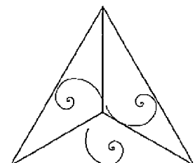
\theta spiral in ELT
