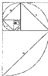
Fibonacci/ \theta spiral
