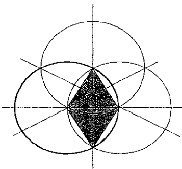
Equilateral romb and rombogram
