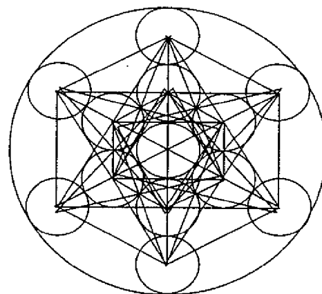
Metatron's cube (Platonic bodies) Constructed from the geometry of the circle
