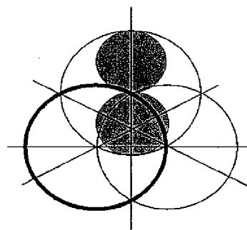
The Ying Yang spiral formed from the geometry of \theta
