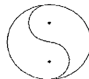
\theta spiral in ELT
