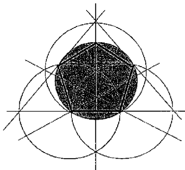
Pentagon and Pentagram
