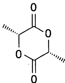
RR or D-lactide
