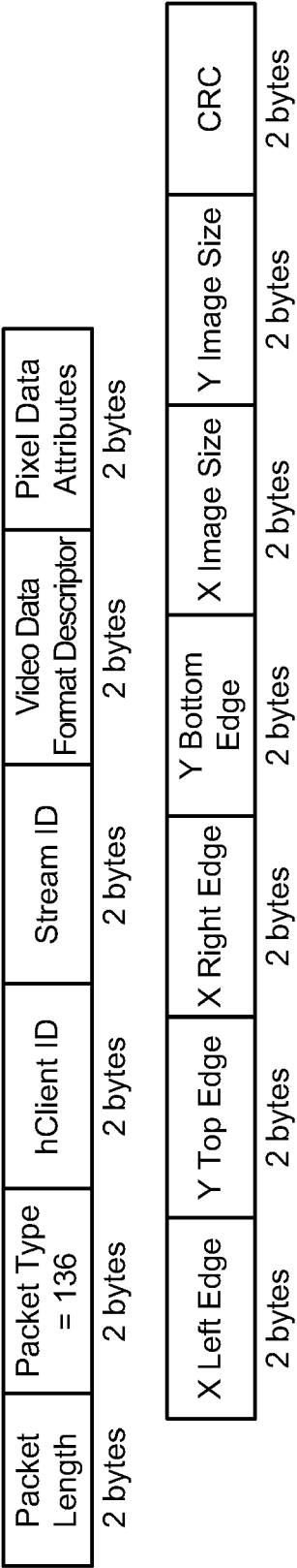
Scaled Video Stream Setup Packet
