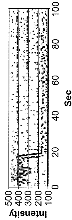
Single Cy3 molecule No free dye in solution
