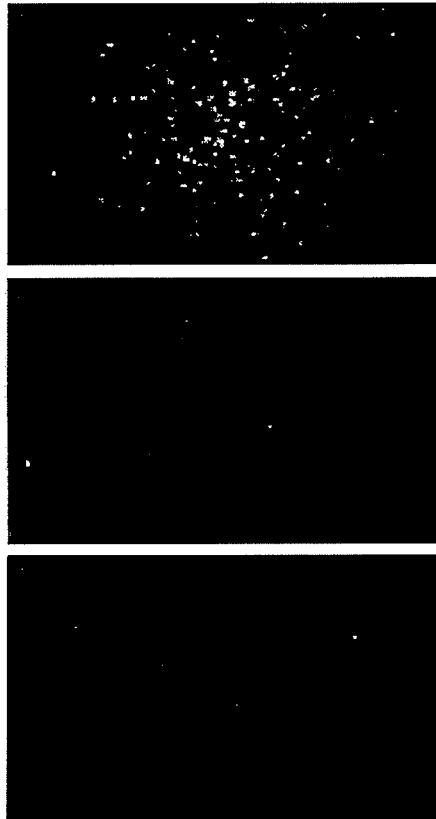
On-surface incorporation in anchored DNA can be visualized at the single-DNA level. (a) Positive incorporation (A-Lis,C,G,T, polymerase). (b) DNA polymerase withheld (A-Lis,C,G,T). (c) Fluorescent nucleotide and DNA polymerase withheld (A,C,G,T).
