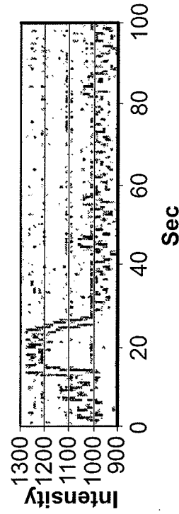
Single Cy3 molecule with background of 15nM Cy3 in solution
