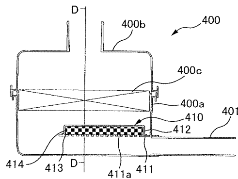
sec C-C FIG. 9B
