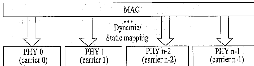
(a) Transmitter
