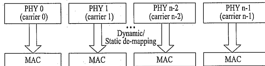
(b) Receiver
