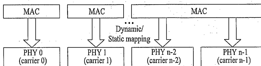
(a) Transmitter
