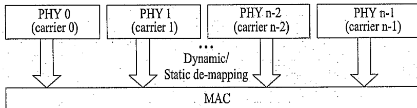
(b) Receiver
