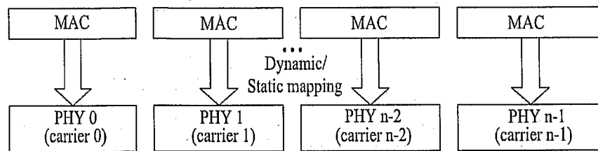
(a) Transmitter
