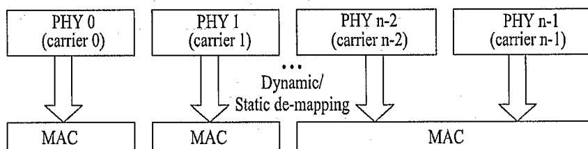
(b) Receiver
