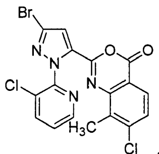
2-[2-Bromo-1-(3-chloro-2-pyridinyl)-1H-pyrazol-5-yl]-7-chloro-8-methyl-4H-3,1-benzoxazine-4-one
