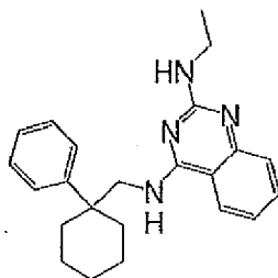
N 2 -ethyl- N 4 -(1-phenyl-cyclohexylmethyl)-quinazoline-2,4-diamine
