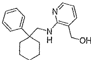
{2-[(1-Phenyl-cyclohexylmethyl)-amino]-pyridin-3-yl}-methanol
