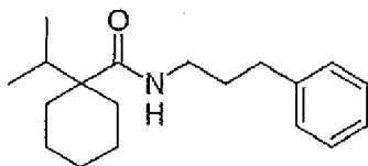
1-Isopropyl-cyclohexanecarboxylic acid (3-phenyl-propyl)-amide
