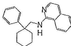
Isoquinolin-1-yl-(1-phenyl-cyclohexylmethyl)-amine
