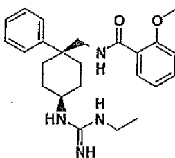
cis-N-[4-(N'-Ethyl-guanidino)-1-phenyl-cyclohexylmethyl]-2-methoxy-benzamide
