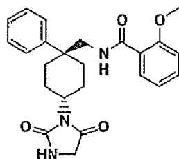
trans-N-[4-(2,5-Dioxo-imidazolin-1-yl)-1-phenyl-cyclohexylmethyl]-2-methoxybenzamide.
