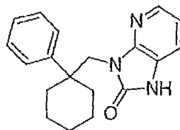
3-(1-Phenyl-cyclohexylmethyl)-1,3-dihydro-imidazo[4,5-b]pyridin-2-one
