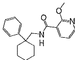
2-Methoxy-N-(1-phenyl-cyclohexylmethyl)-nicotinamide
