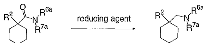
Scheme 20
