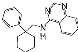
(1-phenyl-cyclohexylmethyl)-quinazolin-4-yl-amine
