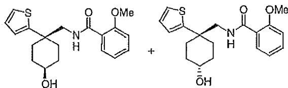
Cis and Trans-N-(4-Hydroxy-1-thiophen-2-yl-cyclohexylmethyl)-2-methoxybenzamide
