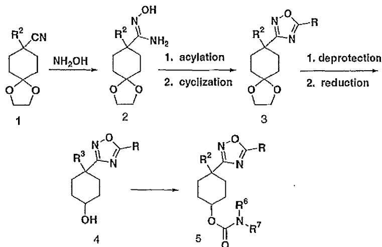
Scheme 12
