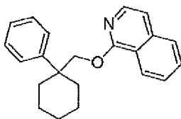
1-(1-Phenyl-cyclohexylmethoxy)-isoquinoline
