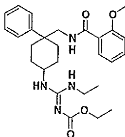
2-Methoxy-N-[4-(N-ethyl-N'-ethoxycarbonyl-guanidino)-1-phenyl-cyclohexylmethyl]-benzamide.
