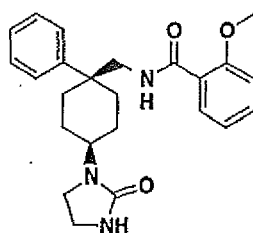
cis-2-Methoxy-N-[4-(2-oxo-imidazolidin-1-yl)-1-phenyl-cyclohexylmethyl]-benzamide
