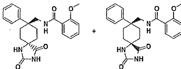
cis- and trans-N-(2,4-Dioxo-1-phenyl-1,3-diaza-spiro[4,5]dec-8-ylmethyl)-2-methoxy-benzamide
