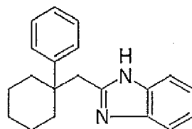
2-(1-Phenyl-cyclohexylmethyl)-1H-benzimidazole
