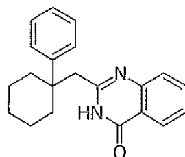
2-(1-Phenyl-cyclohexylmethyl)-3 H -quinazolin-4-one
