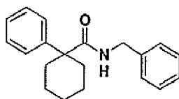
1-Phenyl-cyclohexanecarboxylic acid benzylamide
