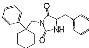
5-Benzyl-3-(1-phenyl-cyclohexylmethyl)-imidazolidine-2,4-dione
