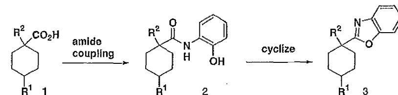
Scheme 15
