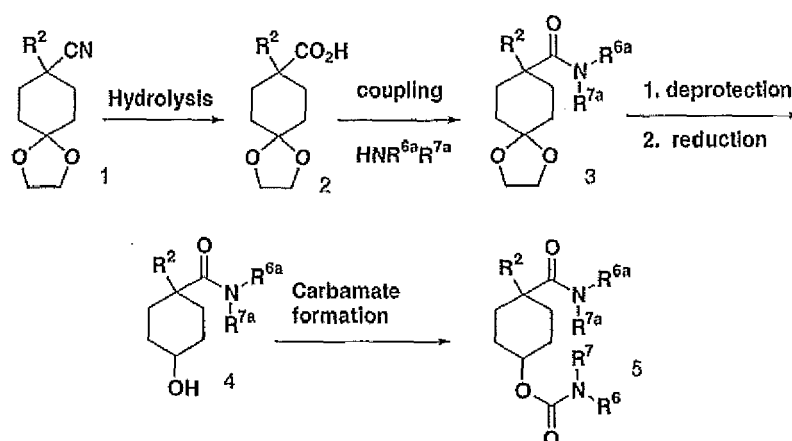
Scheme 17
