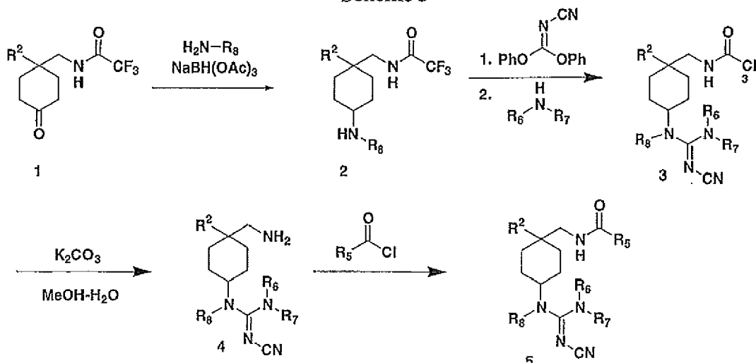
Scheme 3
