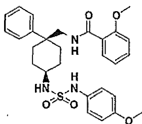
cis-2-Methoxy-N-{4-[N-(4-anisoyl)-N'-sulfenylureido]-1-phenyl-cyclohexylmethyl}-benzamide
