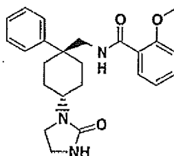
trans-2-Methoxy-N-[4-(2-oxo-imidazolidin-1-yl)-1-phenyl-cyclohexylmethyl]-benzamide
