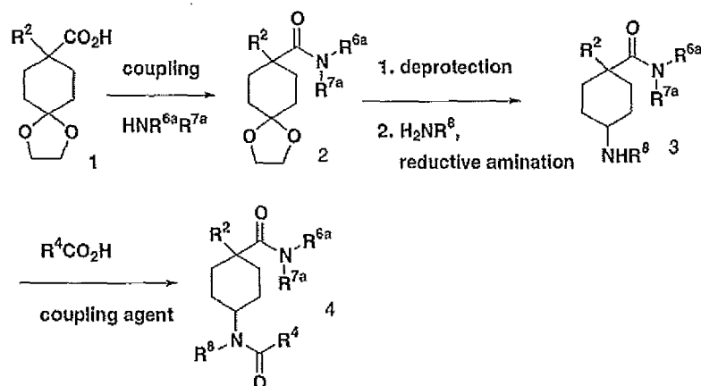
Scheme 18
