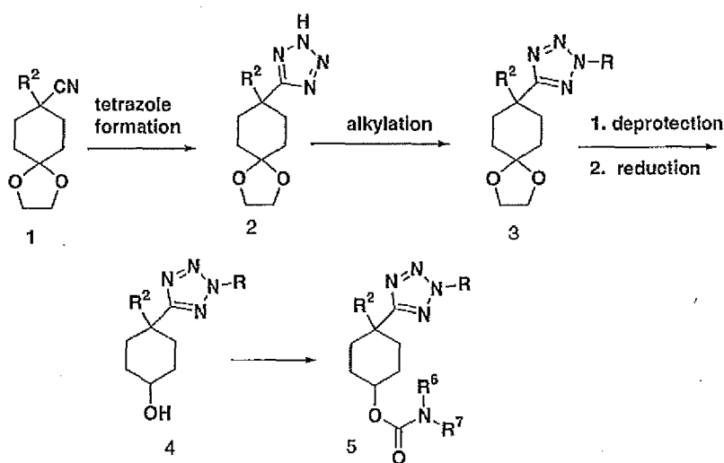
Scheme 13
