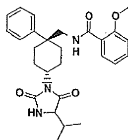
trans-N-[4-(2,5-Dioxo-4-(s)-isopropyl-imidazolin-1-yl)-1-phenyl-cyclohexylmethyl]-2-methoxybenzamide
