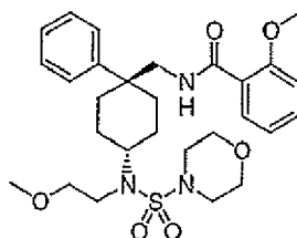
trans-2-Methoxy-N-{4-[(2-methoxy-ethyl)-(morpholine-4-sulfonyl)-amino]-1-phenyl-cyclohexylmethyl}-benzamide
