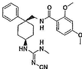
cis-2,4-Dimethoxy-N-[4-(N-methyl-N'-cyanoguanidino)-1-phenyl-cyclohexylmethyl]-benzamide
