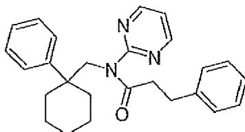
3-Phenyl-N-(1-phenyl-cyclohexylmethyl)-N-pyrimidin-2-yl-propionamide
