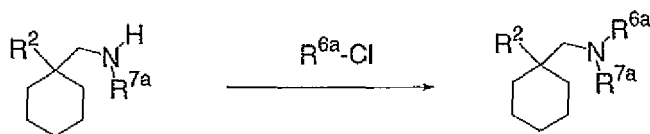
Scheme 21
