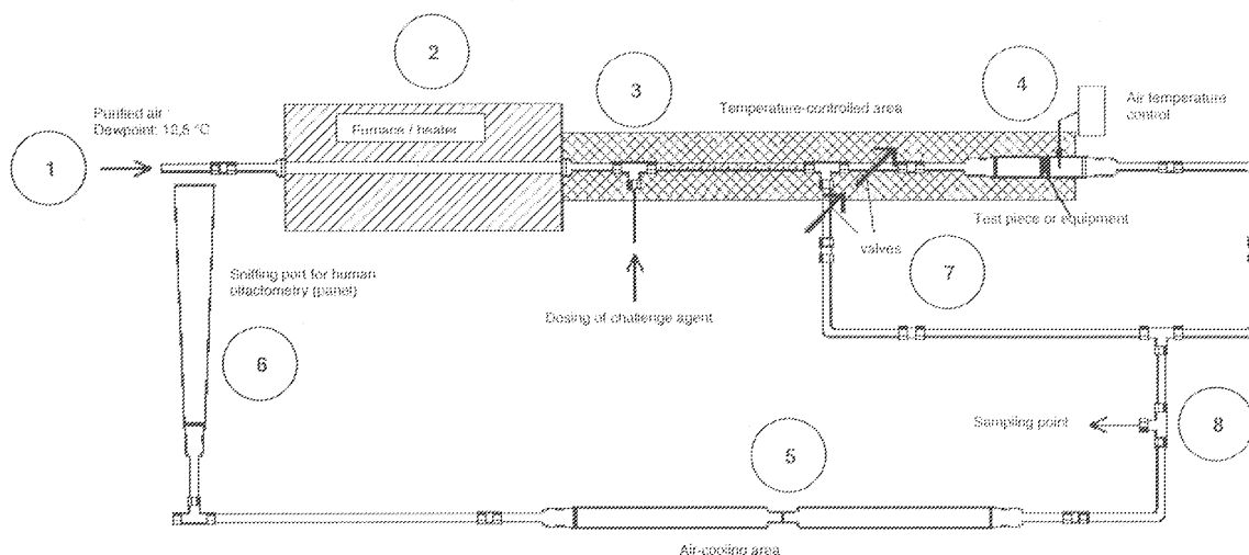
Figure 1 -- Experimental Test Bench
