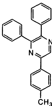
Hdppr-MP
