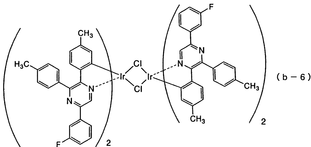
[\text{Ir}(\text{Mdppr-3FP})_2\text{Cl}]_2
