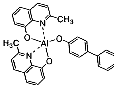
BAQ
