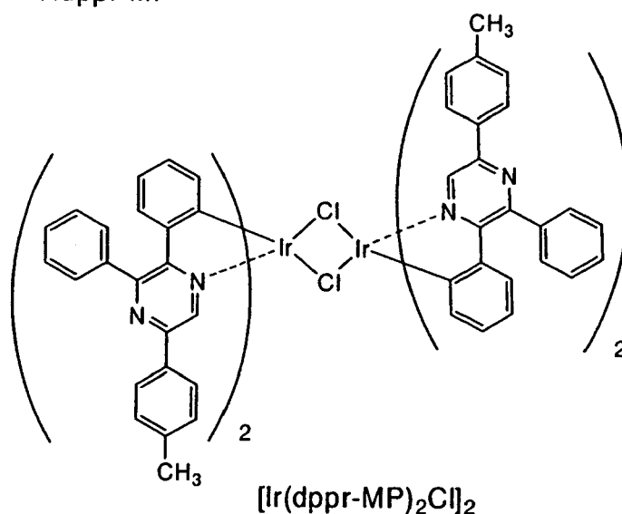
Hdppr-MP
