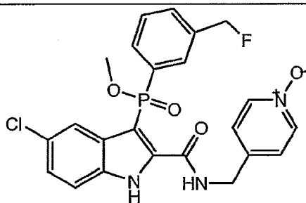
Compound K
