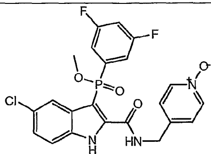
Compound C
