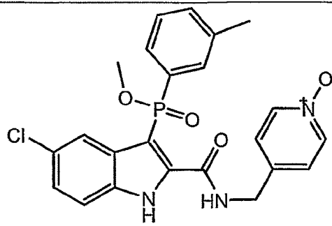
Compound J
