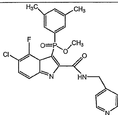
Compound M
