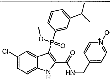
Compound M
