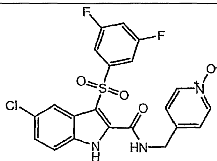
Compound H
