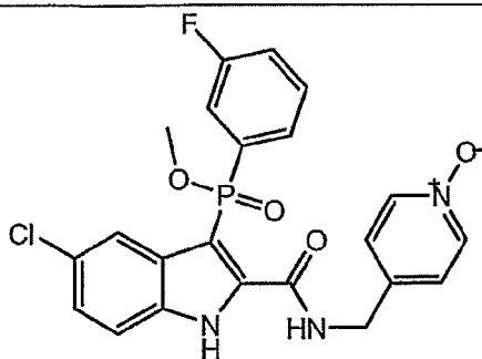
Compound I
