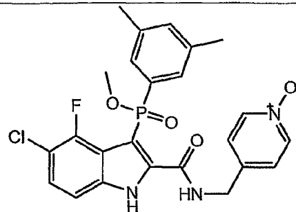
Compound B
