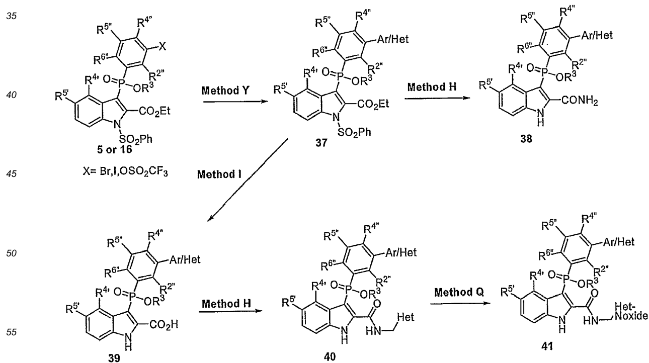
Scheme 10:
