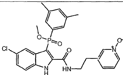
Compound E
