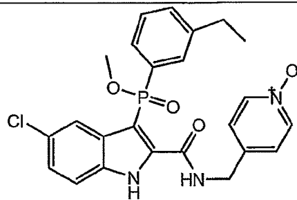
Compound L
