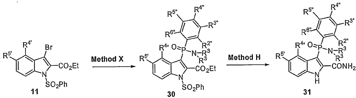
Scheme 8:
