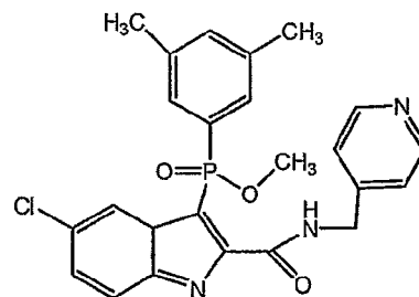
Compound N
