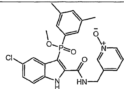
Compound F
