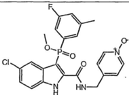
Compound G
