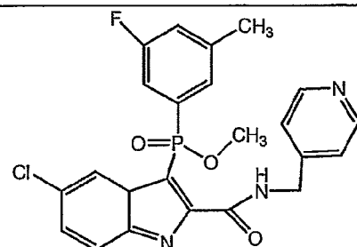
Compound P
