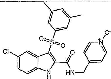
Compound A
