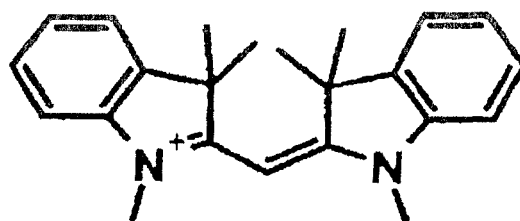
Structural view of cyanine dye
