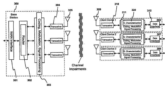
3-Antenna Base Station with 3 Single-Antenna Client Devices
