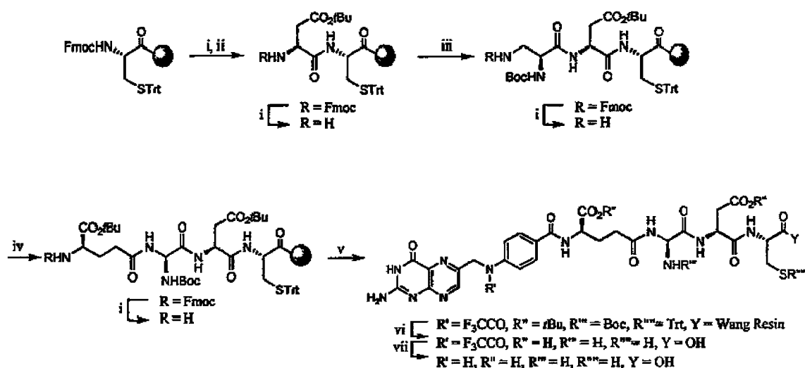
Scheme 1 a
