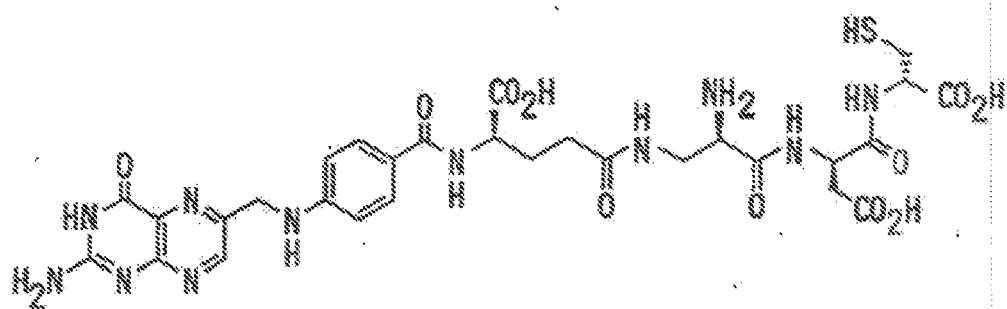
EC53 (Pte-D-γGlu-D-βDpr-D-Asp-D-Cys)
