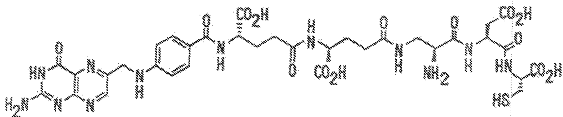
EC11 (Pte-L-γGlu-L-γGlu-L-βDpr-L-Asp-L-Cys)
