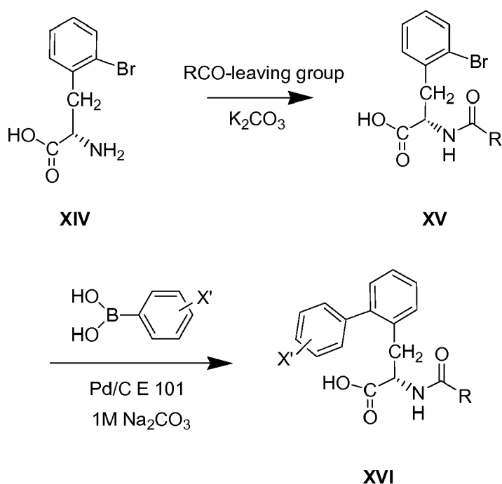
Scheme 3
