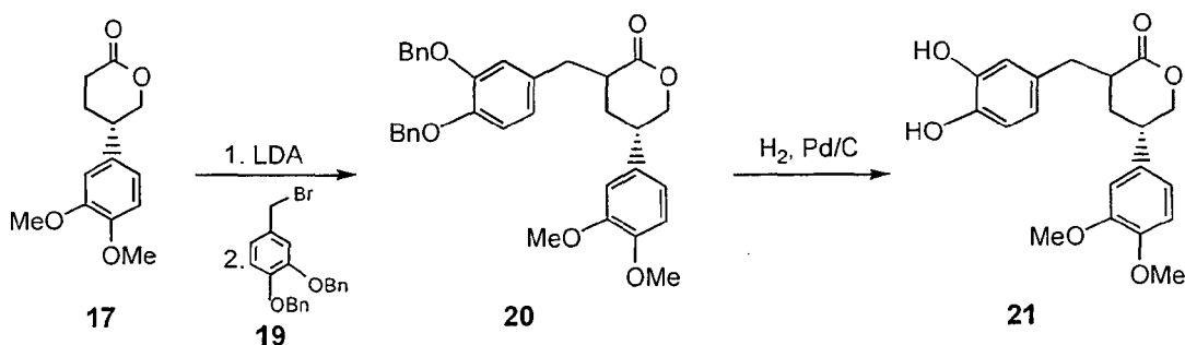
Scheme 5
