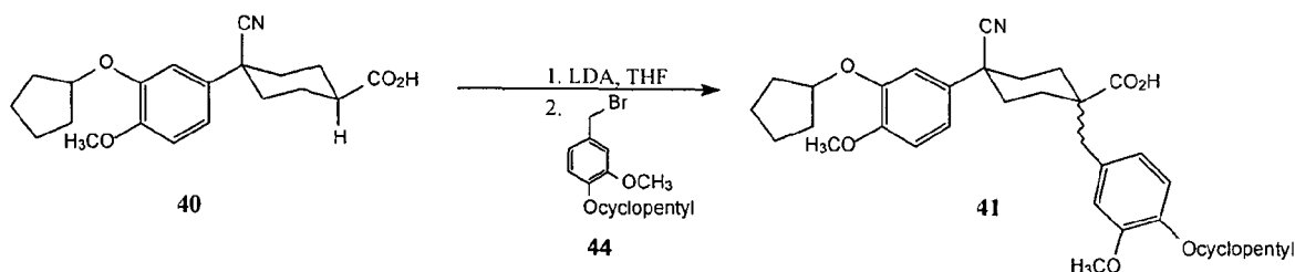
Scheme 10
