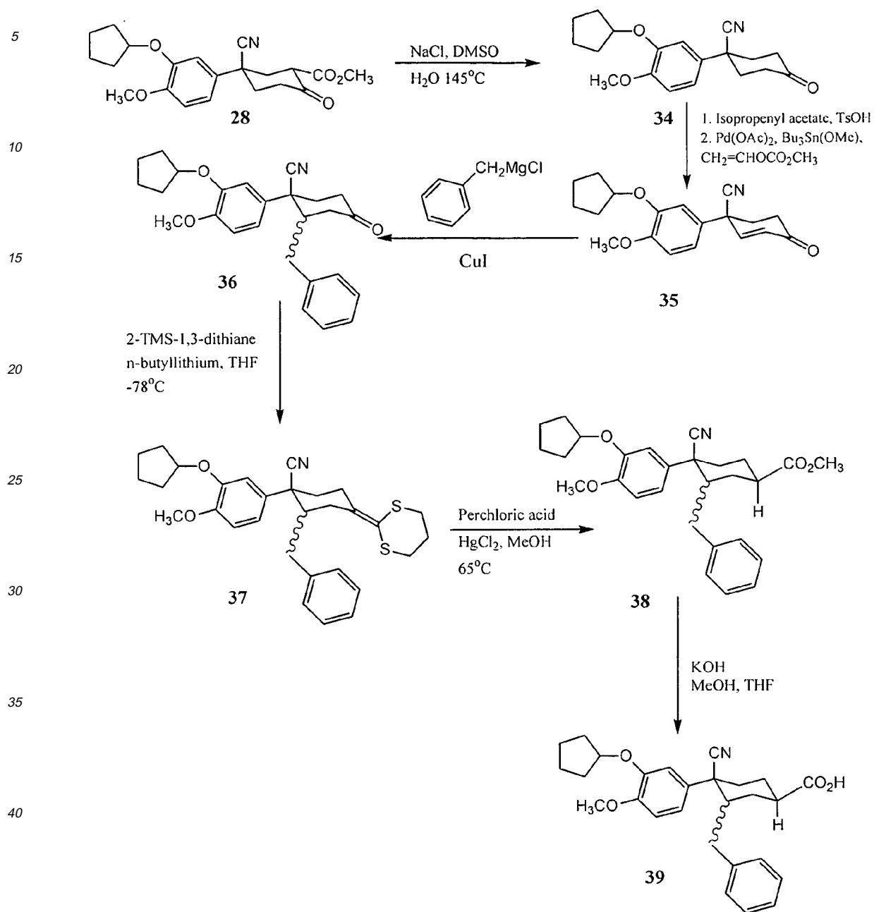
Scheme 9
