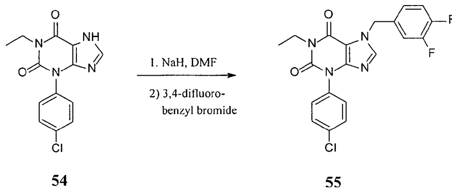
Scheme 16
