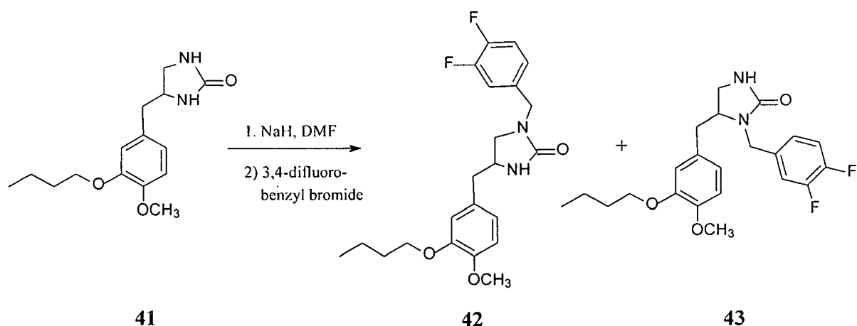
Scheme 13
