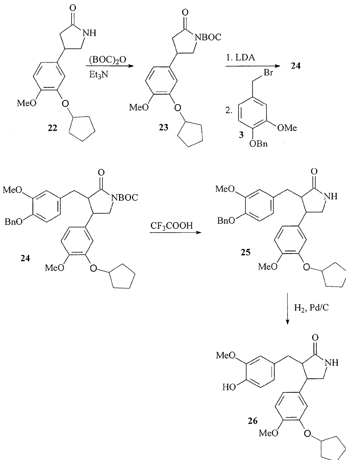
Scheme 6
