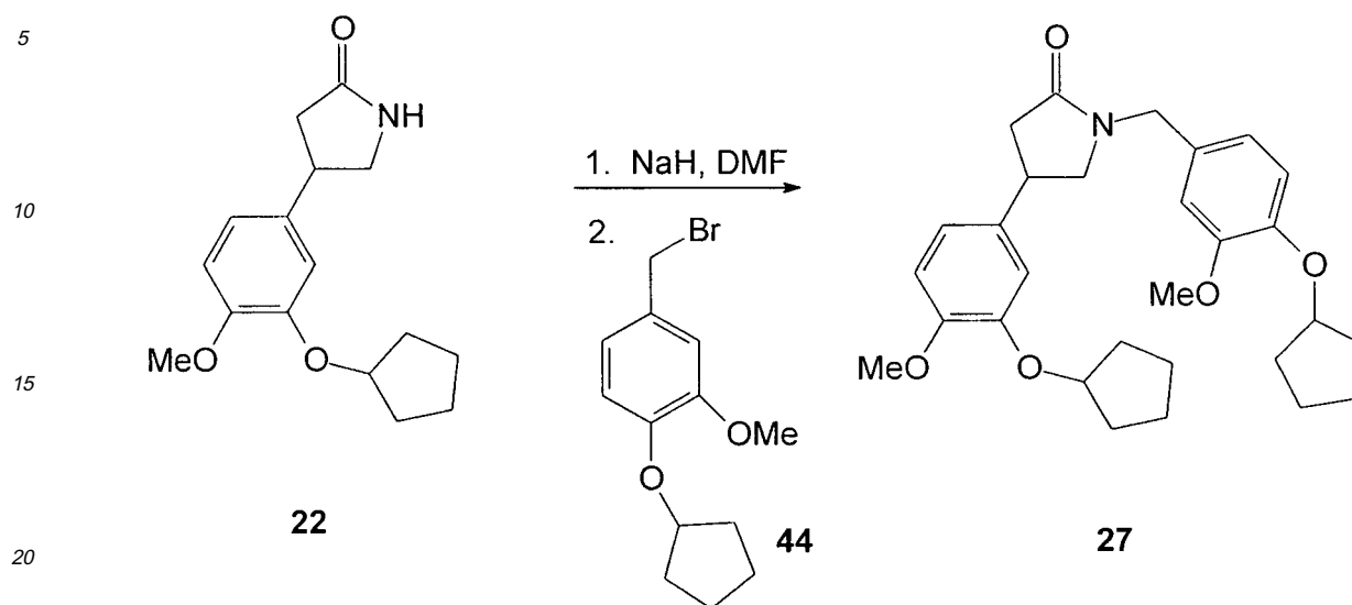
Scheme 7
