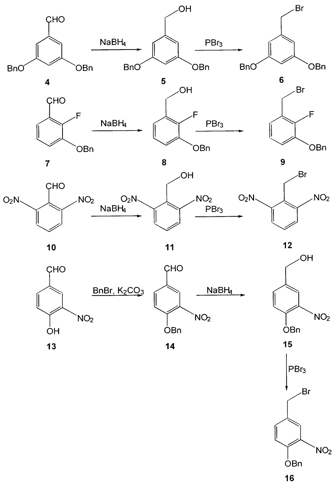
Scheme 3
