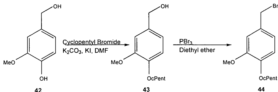
Scheme 11
