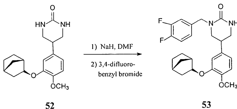
Scheme 15
