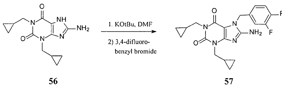
Scheme 17
