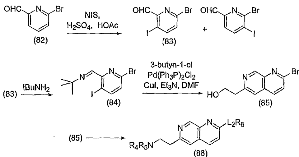
Scheme 16
