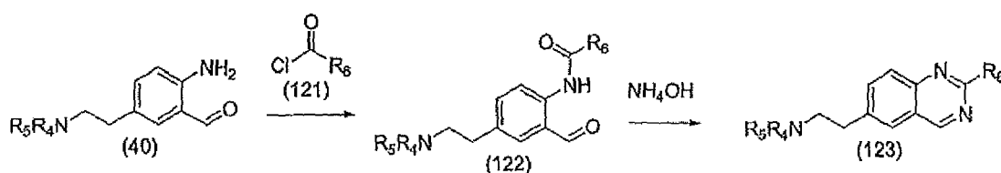
Scheme 22
