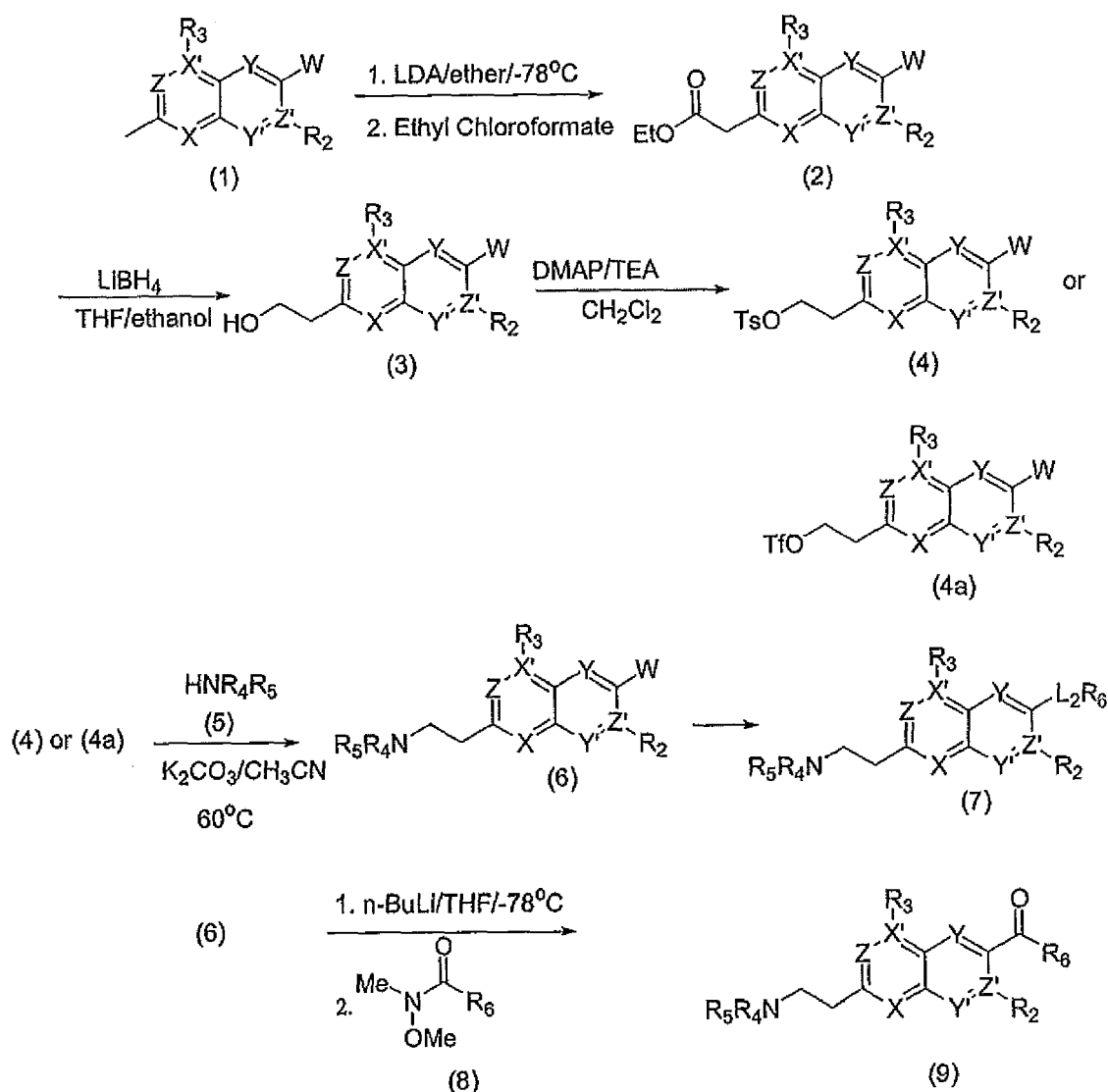
Scheme 1
