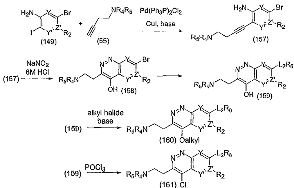
Scheme 26
