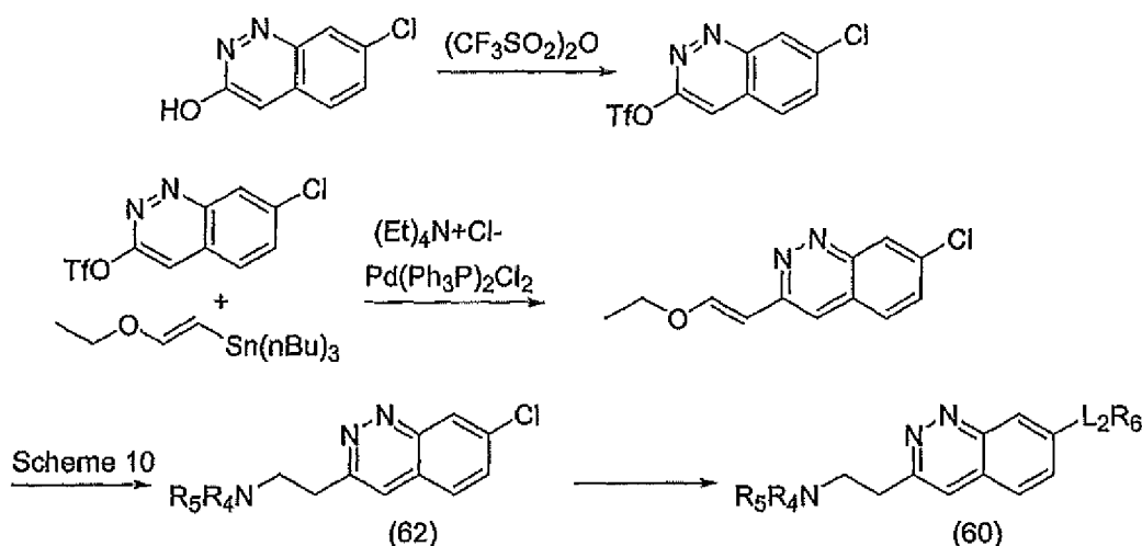
Scheme 12
