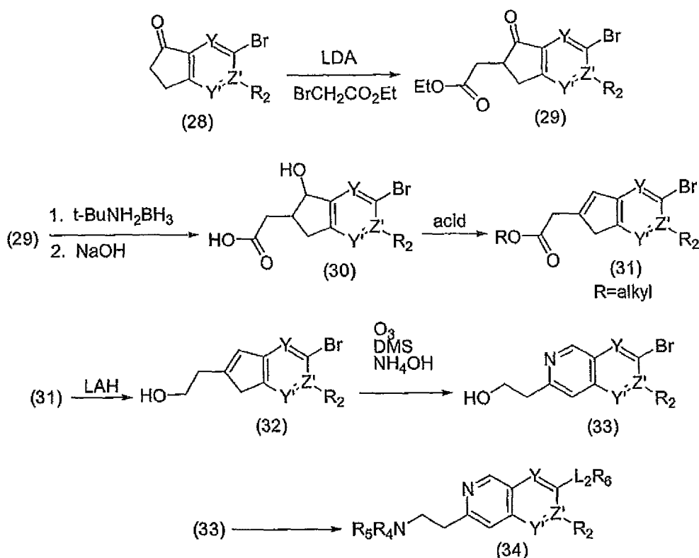
Scheme 7
