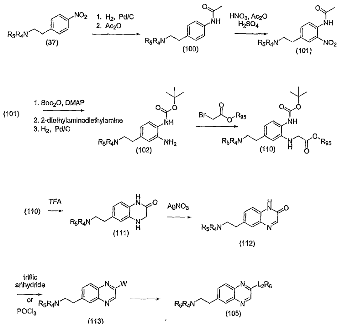
Scheme 20
