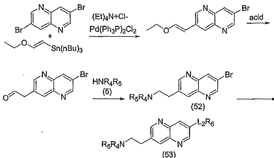
Scheme 10
