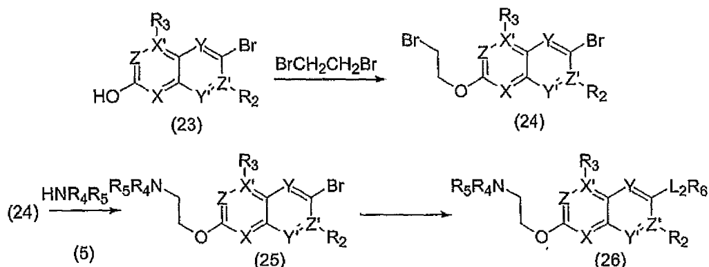
Scheme 6
