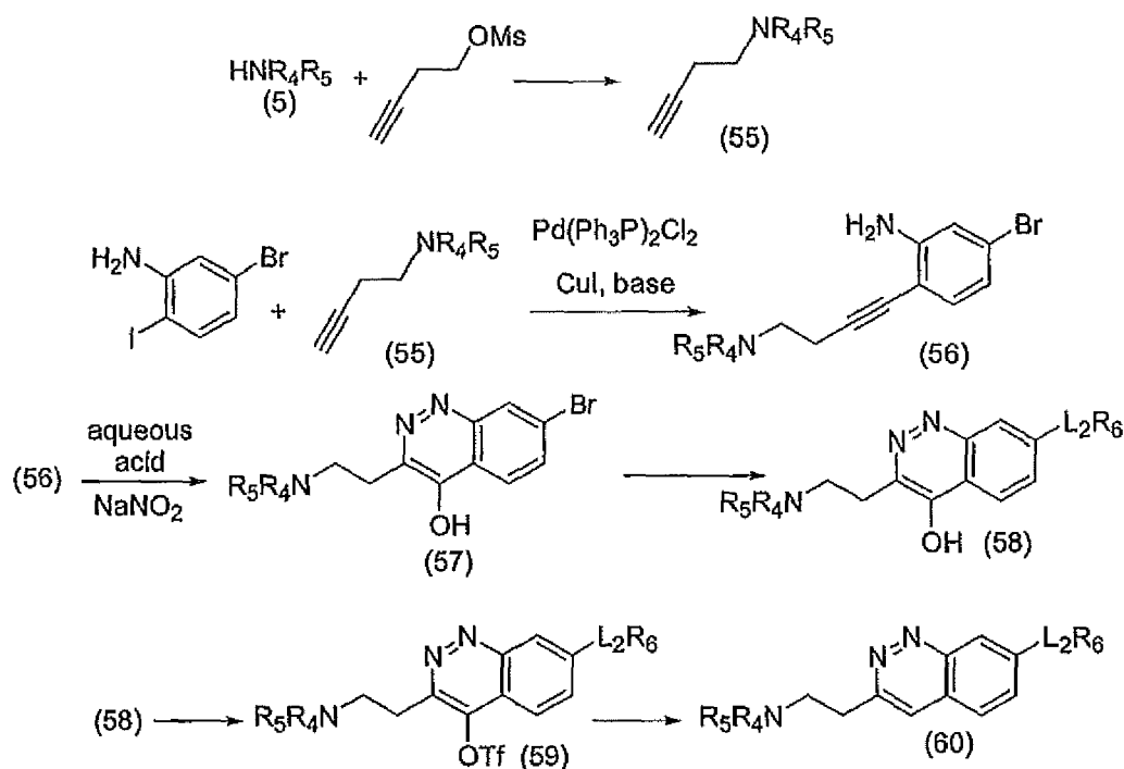
Scheme 11
