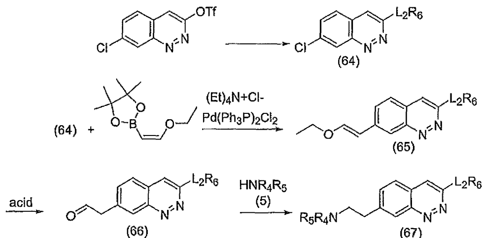
Scheme 13
