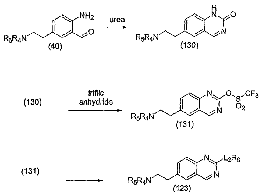
Scheme 23
