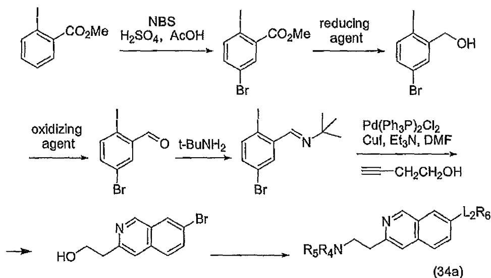
Scheme 19
