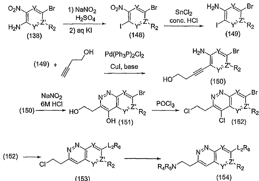
Scheme 25
