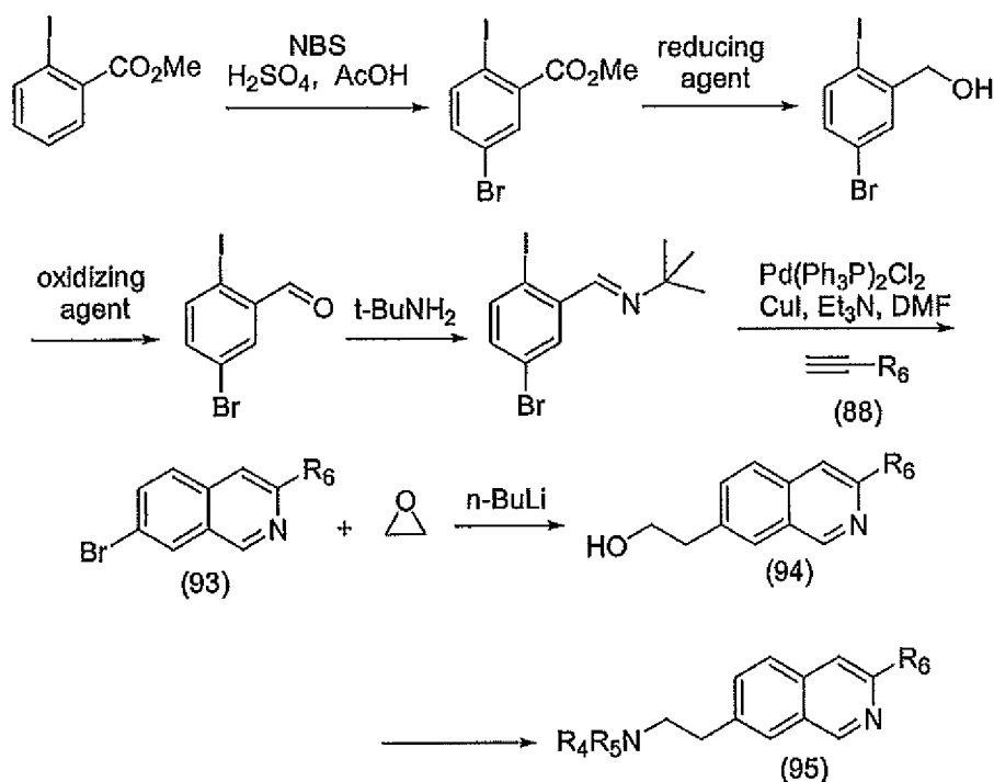
Scheme 18
