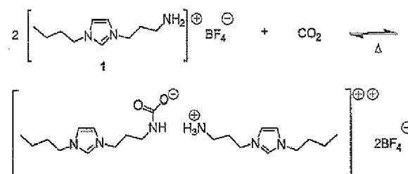
Scheme 2. Proposed reaction between TSIL 1 and CO 2 .
