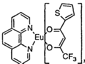
Eu(TTA) 3 phen
