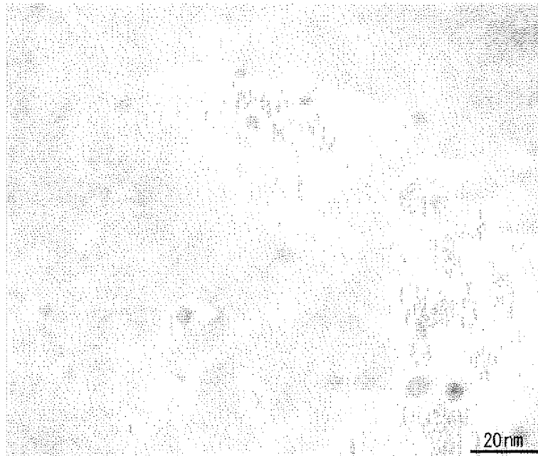
Alloy No. 11 Transmission Electron Image of Precipitated Grains after Heating at 700° C for 120 seconds in Compression-Processed Material in Process K0 Average Grain Diameter 4.6 mm
