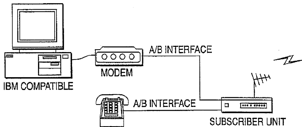
POTS TERMINAL INTERFACE FIG. 2B
