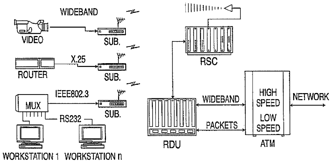
WIDEBAND AND PACKET NETWORK INTERFACE
