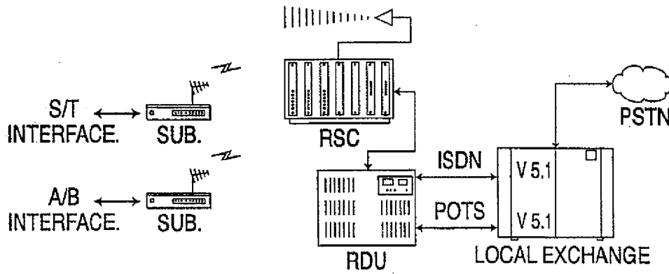
ISDN AND POTS NETWORK INTERFACE
