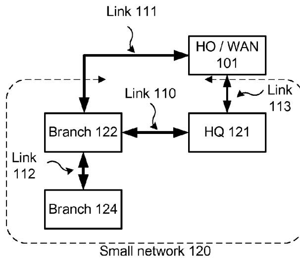
Fig. 1b: A Small Network – Connection Diagram
