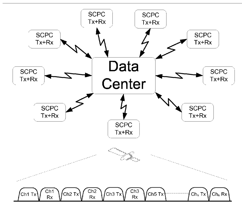
Fig. 8d: SCPC Topology PRIOR ART
