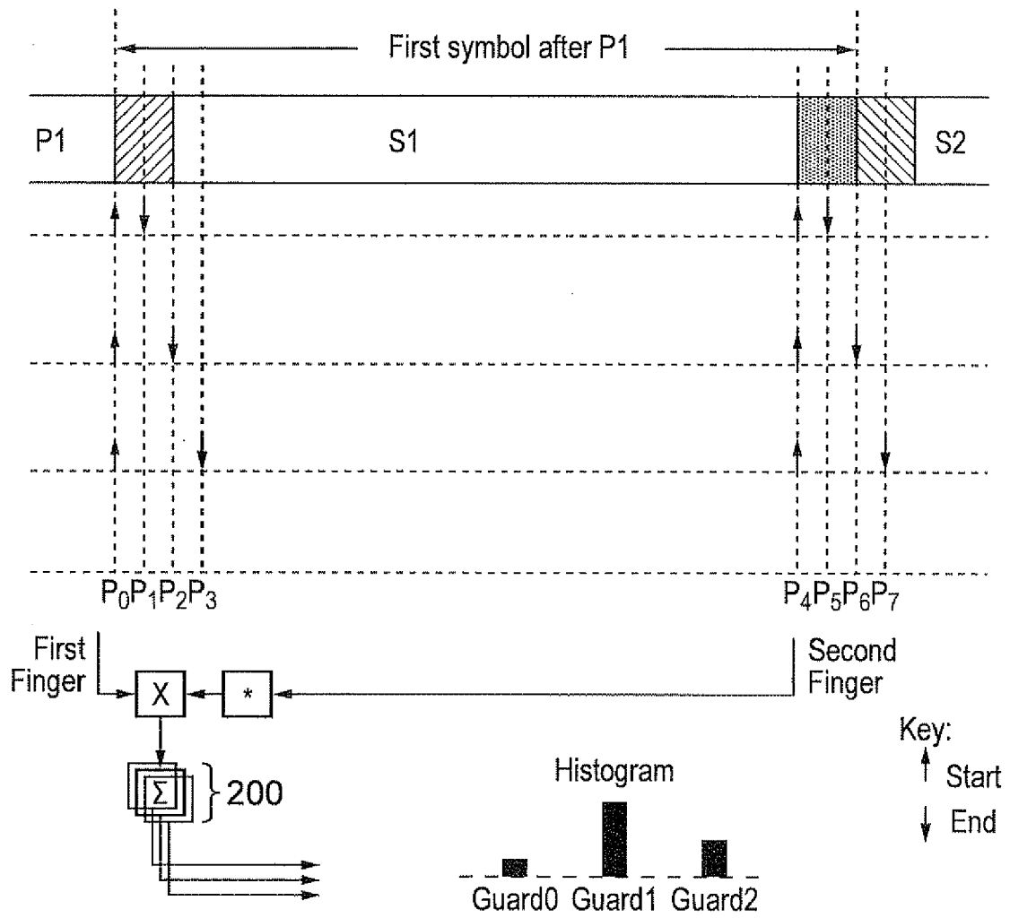
Operation of Simplified Architecture at First Symbol
