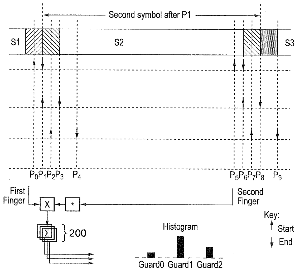
Operation of Simplified Architecture at Second Symbol
