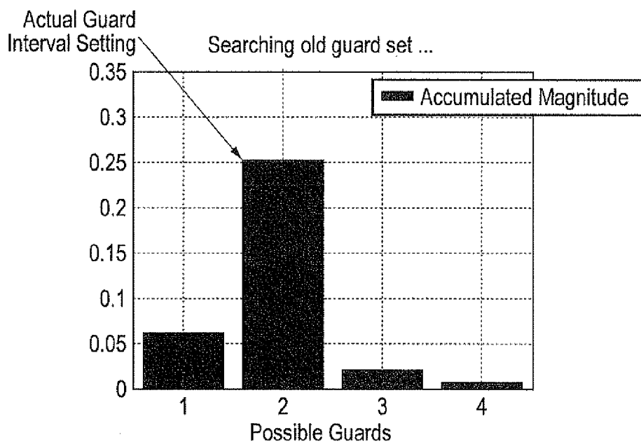
'Accumulated Correlation Magnitudes' for Possible Guard Intervals
