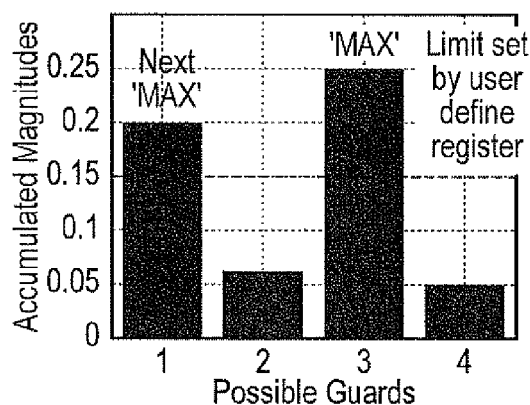
'Accumulated Correlation Magnitudes' for Possible Guard Intervals
