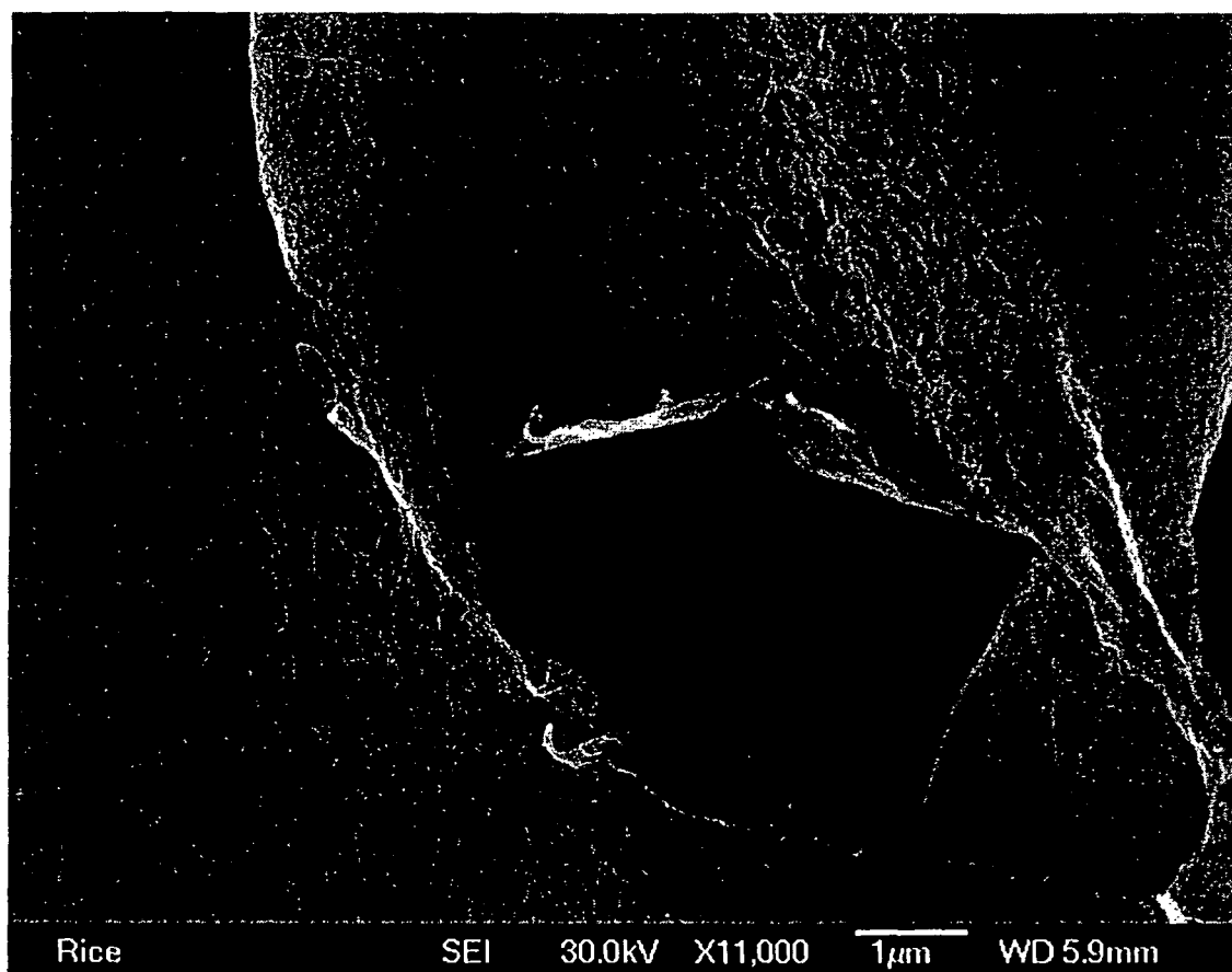
Figure 29: Thin silica-SWNT paper formed by light etching of coated nanotubes.
