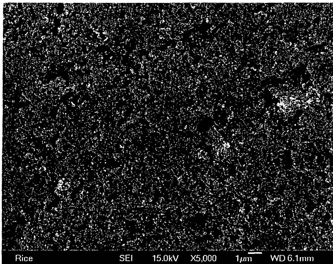
Figure 6: SEM image, at 5,000x, of product of LPD silica reaction with fulleranol added to reaction mixture.
