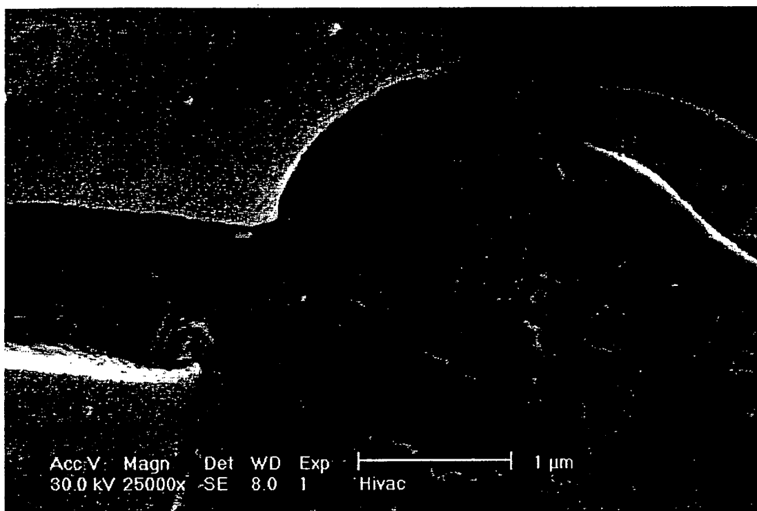
Figure 21: SEM image, at 25,000x, of the product of the reaction of SDS dispersed SWNTs with the LPD silica solution.
