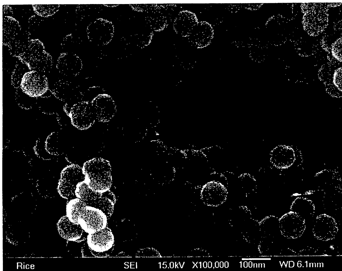
Figure 7: SEM image, at 100,000x, of product of LPD silica reaction with fullereneol added to reaction mixture.
