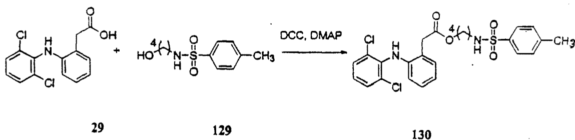
Scheme 22
