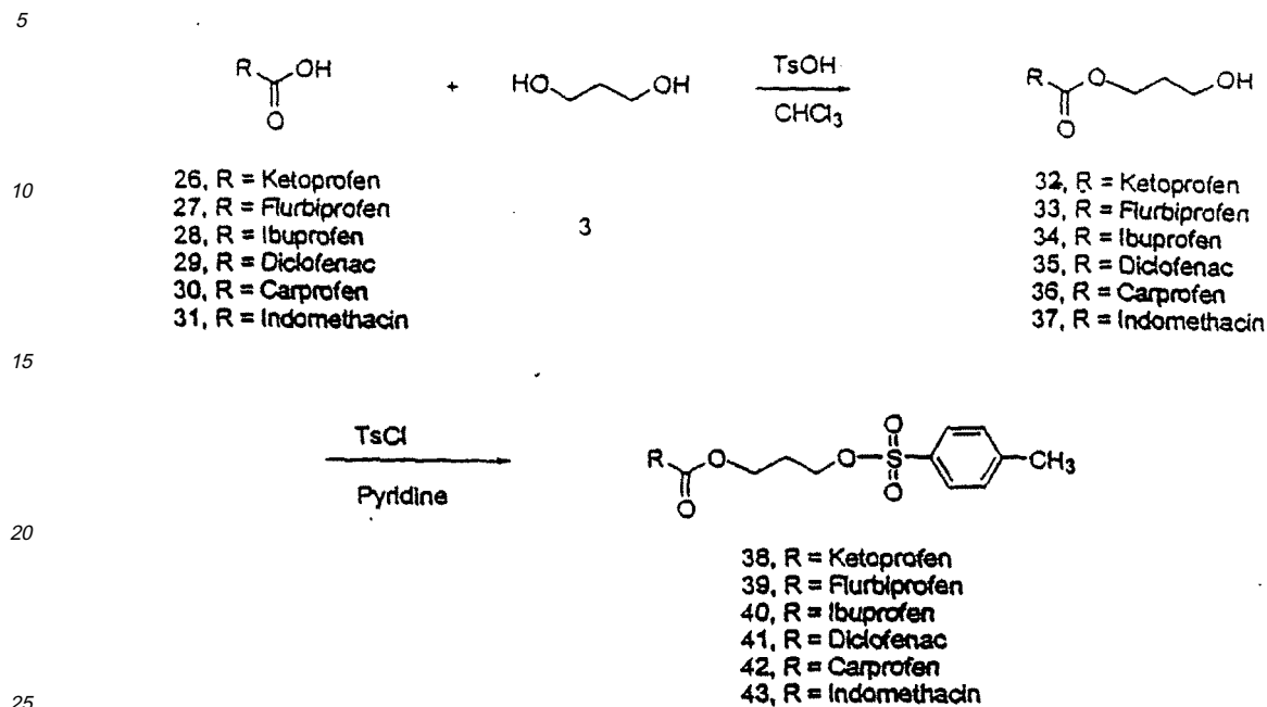
Scheme 3
