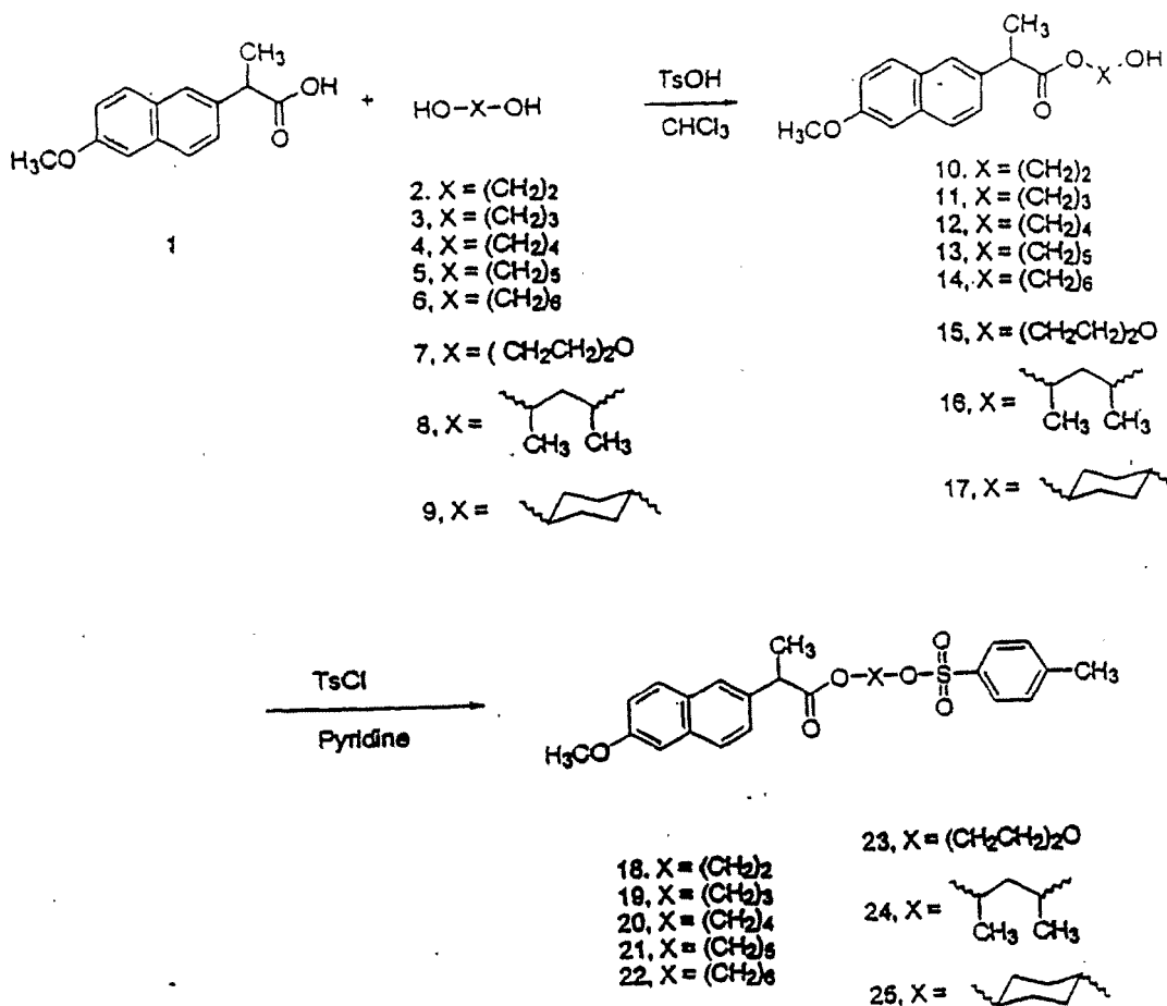
Scheme 2
