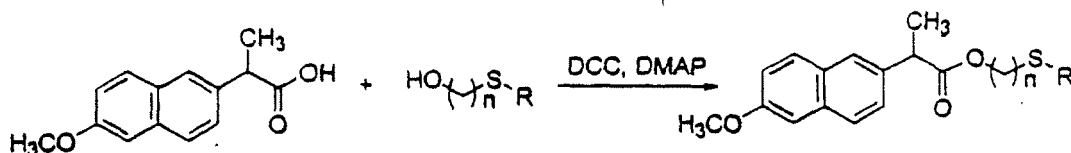
Scheme 13
