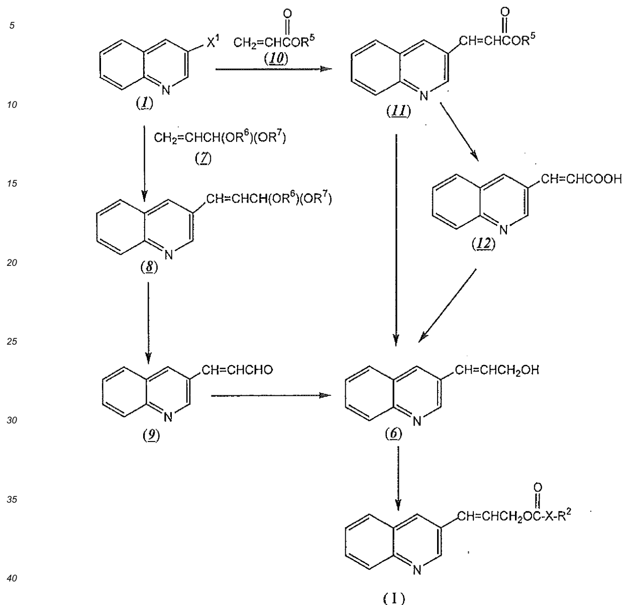
Scheme 4
