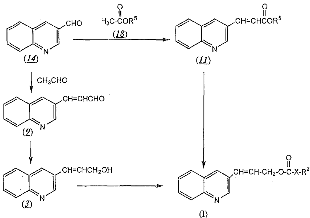
Scheme 7
