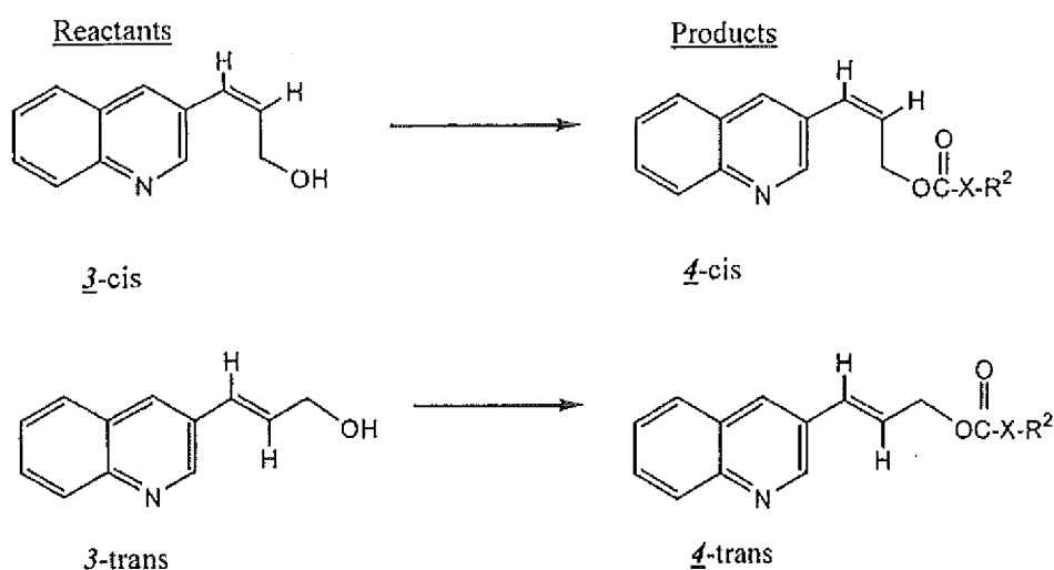
Scheme 3
