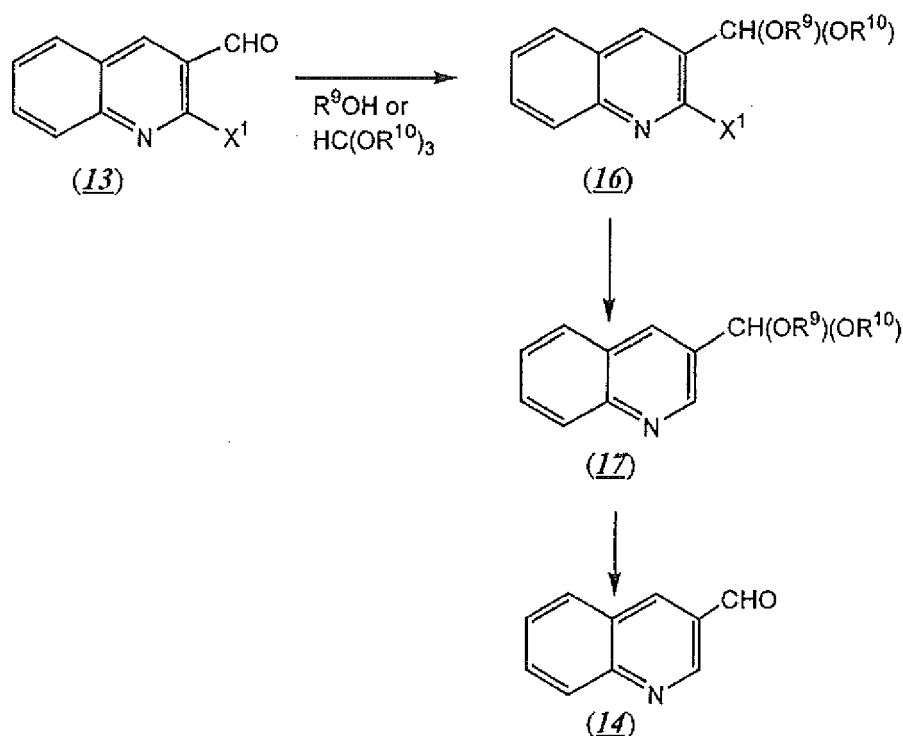
Scheme 6
