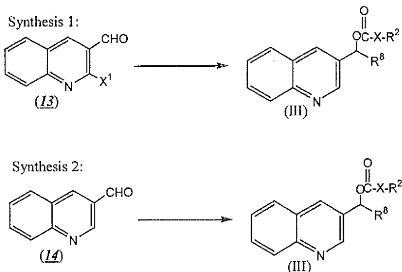
Scheme 5
