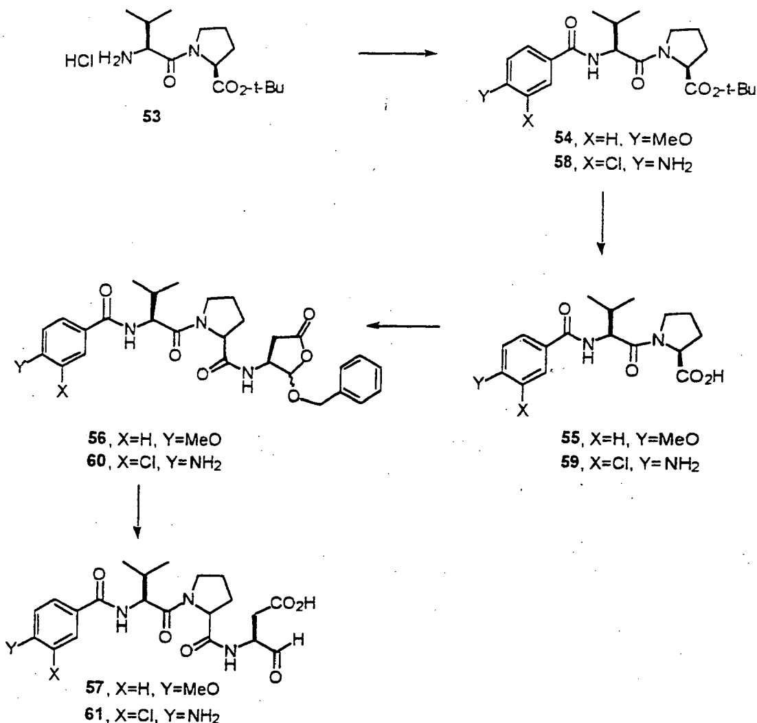
Scheme XII
