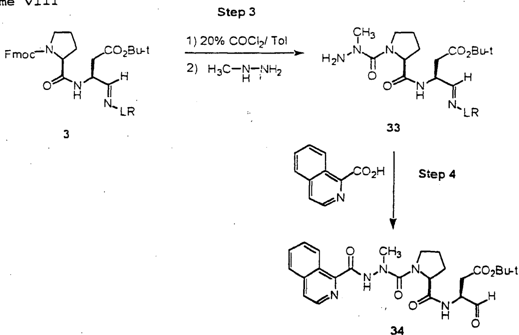
Scheme VIII
