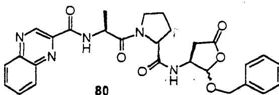
Quinoxaline-2-carboxylic acid {2-[2-(2-benzyloxy-5-oxo-tetrahydrofuran-3-ylcarbamoyl)-pyrrolidin-1-yl]-1-methyl-2-oxo-ethyl}-amide (80).
