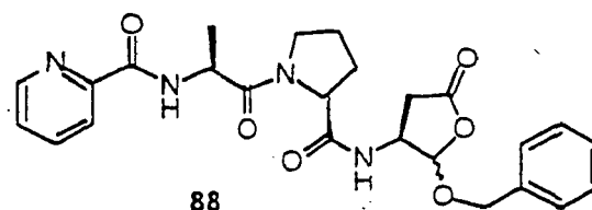
Pyridine-2-carboxylic acid{2-[2-(2-benzyloxy-5-oxo-tetrahydro-furan-3-ylcarbamoyl)-pyrrolidin-1-yl]-1-methyl-2-oxo-ethyl}-amide (88).
