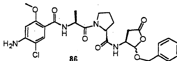
1-[2-(4-Amino-5-chloro-2-methoxy-benzoylamino)-propionyl]-pyrrolidine-2-carboxylic acid (2-benzyloxy-5-oxo-tetrahydro-furan-3-yl)-amide (86).
