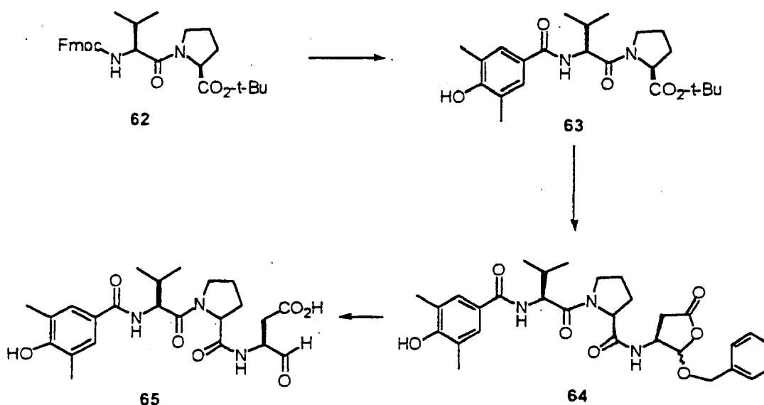
Scheme XIII
