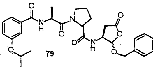
1-[2-(3-Isopropoxy-benzoylamino)-propionyl]-pyrrolidine-2-carboxylic acid (2-benzyloxy-5-oxo-tetrahydro-furan-3-yl)-amide (79).
