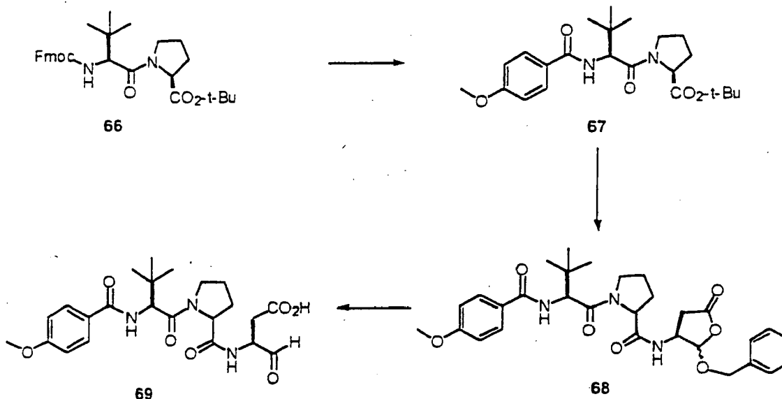
Scheme XIV
