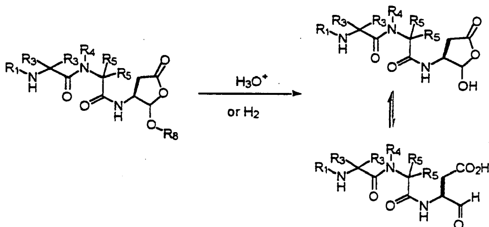
Scheme XXIII
