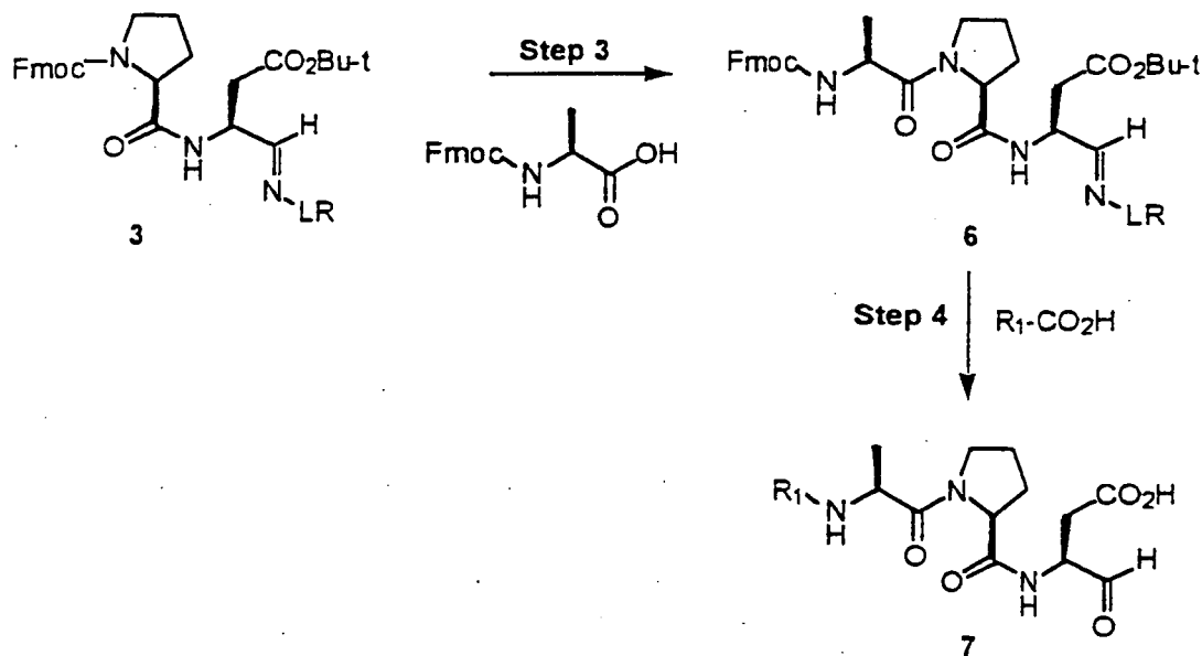
Scheme II
