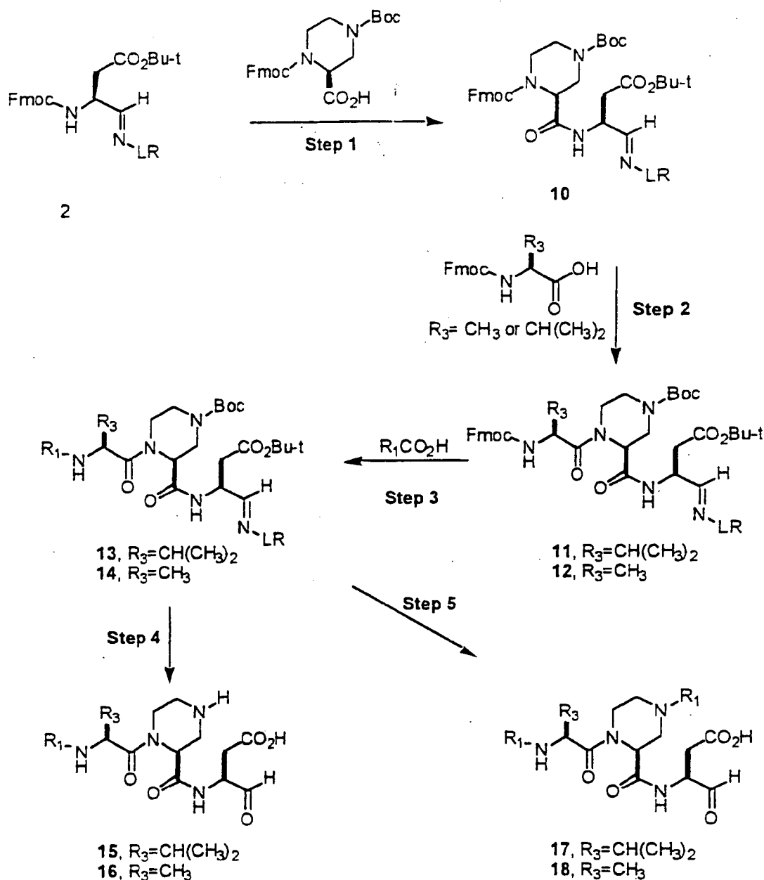
Scheme IV
