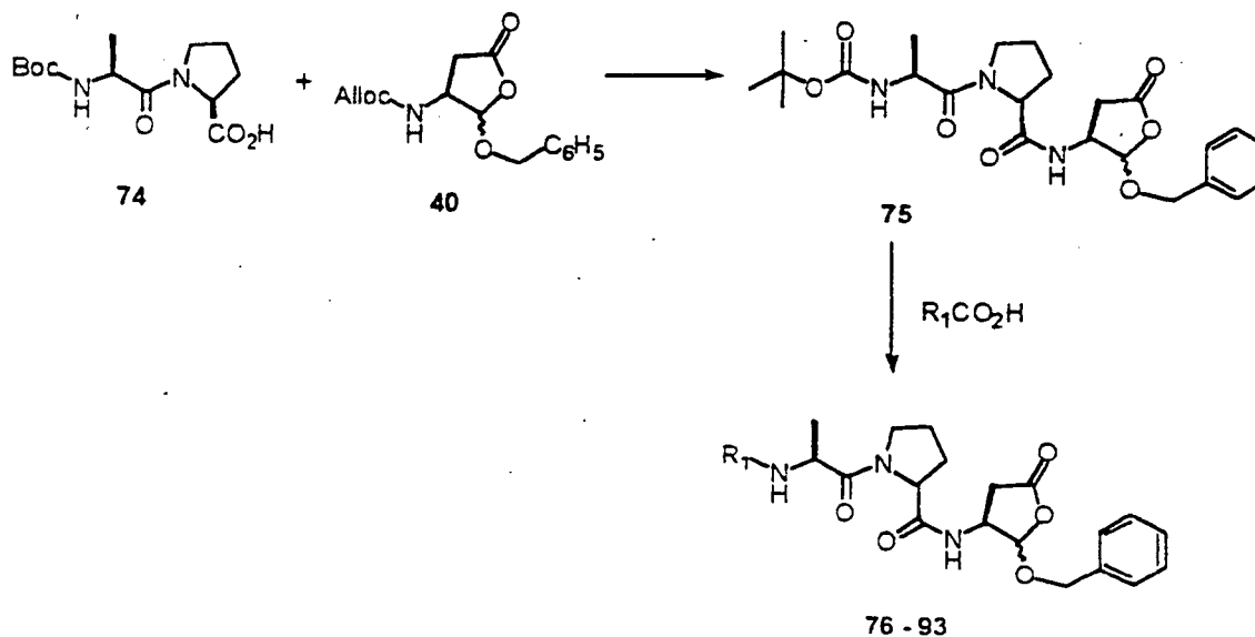
Scheme XVI
