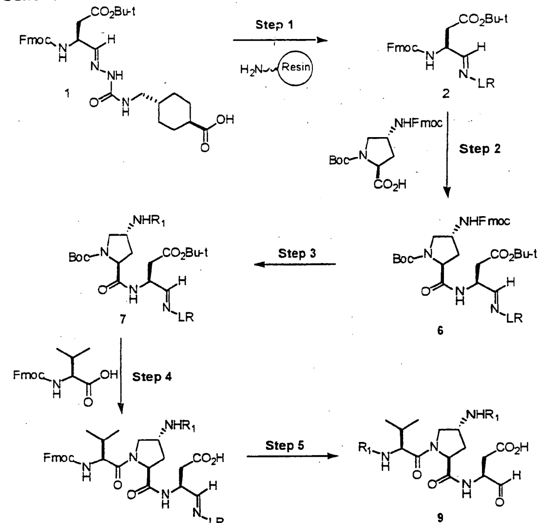
Scheme III
