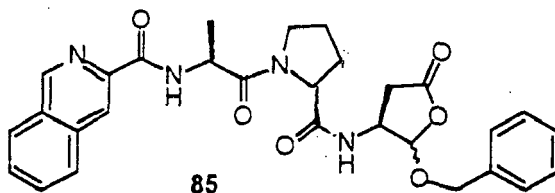
Isoquinoline-1-carboxylic acid {2-(2-benzyloxy-5-oxo-tetrahydro-furan-3-ylcarbamoyl)-pyrrolidin-1-yl}-1-methyl-2-oxo-ethyl)-amide (85).
