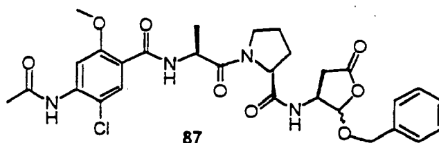
1-[2-(4-Acetylamino-5-chloro-2-methoxy-benzoylamino)-propionyl]-pyrrolidine-2-carboxylic acid (2-benzyloxy-5-oxo-tetrahydro-furan-3-yl)-amide (87).
