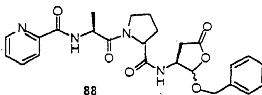
Pyridine-2-carboxylic acid{2-[2-(2-benzyloxy-5-oxotetrahydro-furan-3-ylcarbamo-yl)-pyrrolidin-1-yl]-1-methyl-2-oxo-ethyl}-amide (88).
