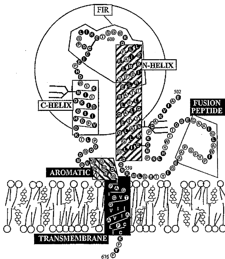
Ebola virus GP2 Figure 4
