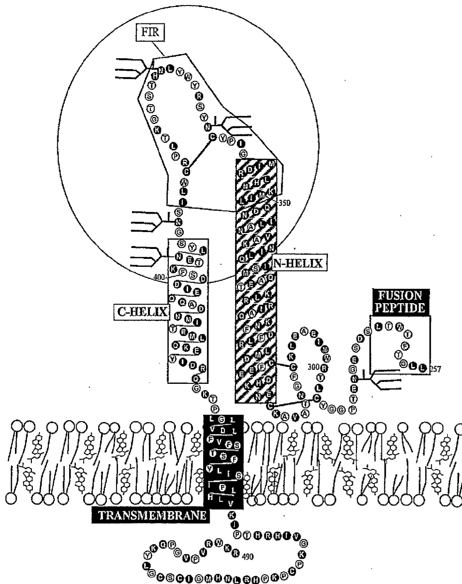
Lassa virus GP2 Figure 2
