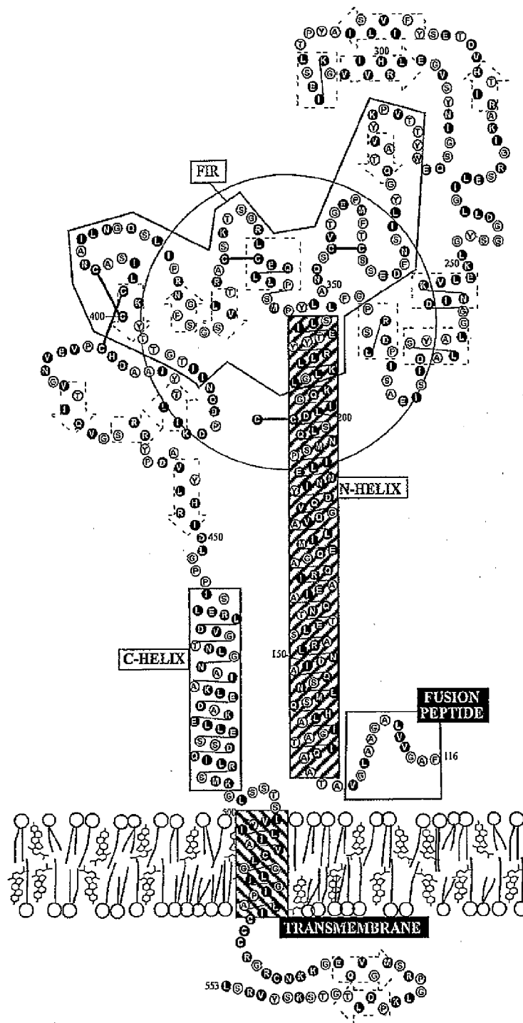
measles virus F1 Figure 6
