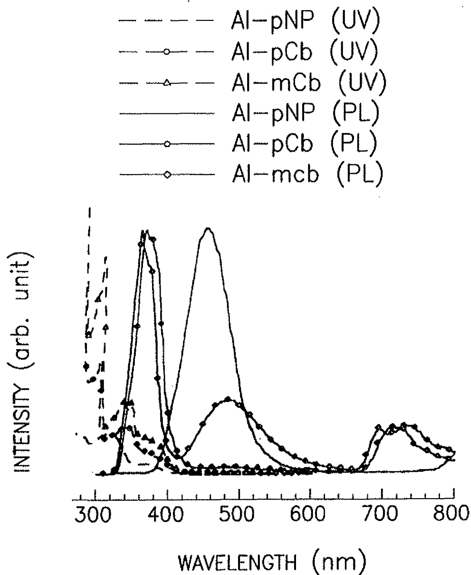
Absorption and Fluorescent Spectra of Al-pNP, Al-pCb, and Al-mCb in \text{CH}_2\text{Cl}_2 Solution
